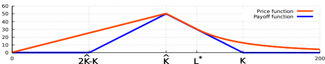
Fig. S.74: American butterfly payoff and price functions.
