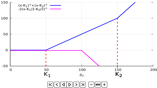
Fig. S.27: Butterfly option as a combination of call options.*
