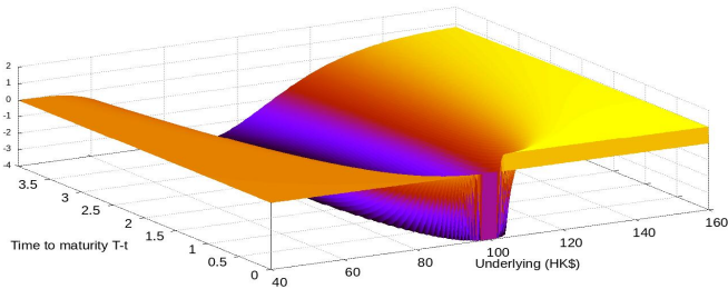
Fig. S.33: Risk-free hedging portfolio value for a binary call option.
