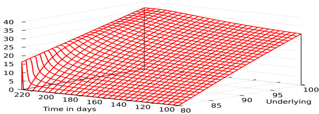
Fig. S.54: Price of the down-and-out long forward contract with K = 60 < B = 80 .
