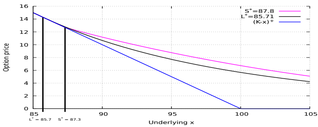
Fig. S.75: Perpetual vs finite expiration American put option price.
