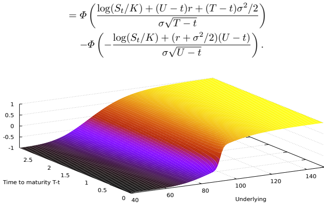
Fig. S.35: Delta of the maximum chooser option.
