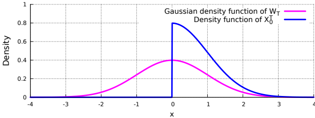
Fig. 10.9: Probability density of the maximum X_0^1 of Brownian motion over [0, 1] .
