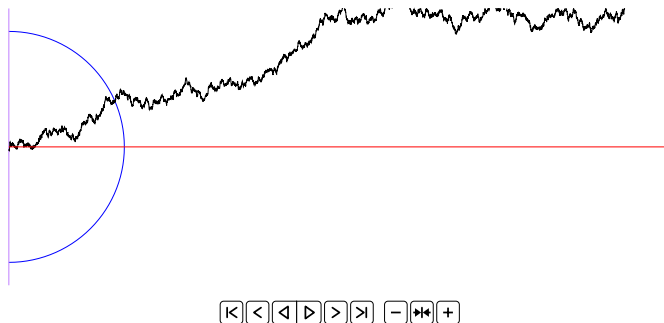
Fig. 10.3: Zeroes of Brownian motion.*
