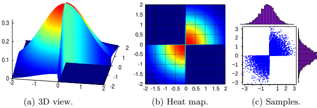
Fig. 4.11: Truncated two-dimensional Gaussian density.
