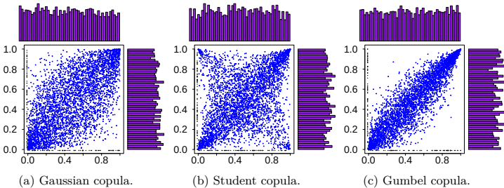
Fig. 4.6: Samples with uniform marginals and given copulas.
