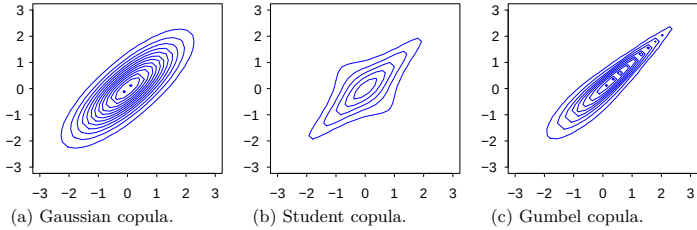
Fig. 4.9: Joint density contour plots with Gaussian marginals and given copulas.
