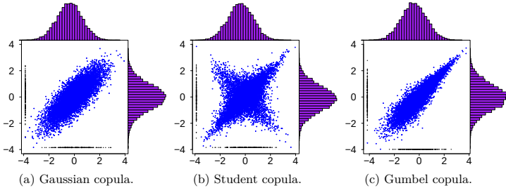
Fig. 4.7: Samples with Gaussian marginals and given copulas.
