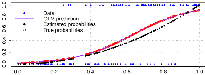
Fig. 11.7: GLM regression.
