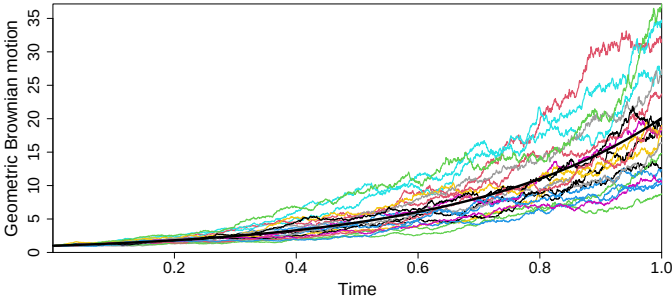
Fig. S.1: Twenty sample paths of geometric Brownian motion (S_t)_{t \in \mathbb{R}_+} .
