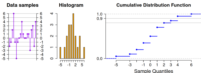
Fig. 7.8: Data set and cumulative distribution function.
