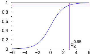
(a) Logistic quantile and CDF.
