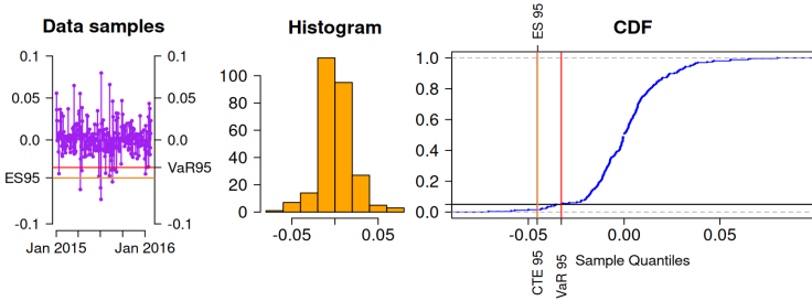
Fig. 7.3: Value at Risk and Expected Shortfall.
