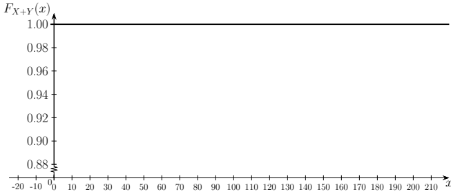
Fig. 7.11: Cumulative distribution function of X + Y .
