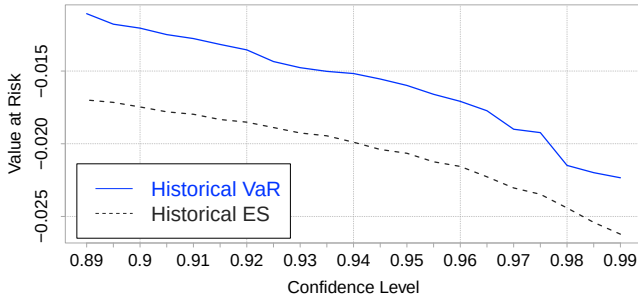
Fig. 7.4: Value at Risk vs. Expected Shortfall.
