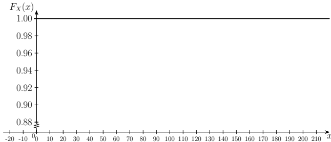
Fig. 7.10: Cumulative distribution function of X .
