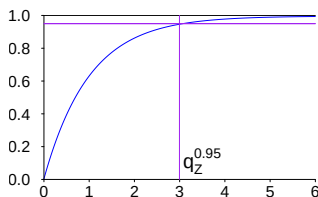
(a) Exponential quantile and CDF.
