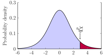
(b) Logistic PDF.
