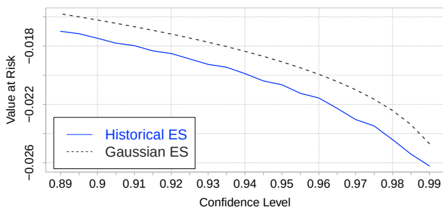
Fig. 7.6: Historical vs. Gaussian estimates of Expected Shortfall.
