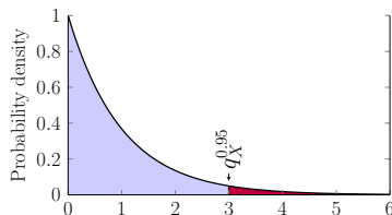
(b) Exponential PDF.
