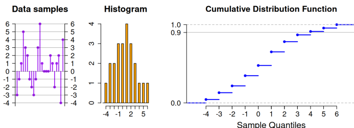
Fig. 7.9: Data set and cumulative distribution function.
