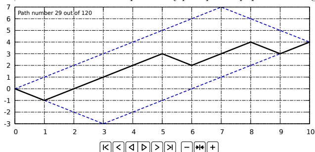
Fig. 1.2: Graph of 120 = \binom{10}{7} = \binom{10}{3} paths with n = 5 and k = 2 .*
