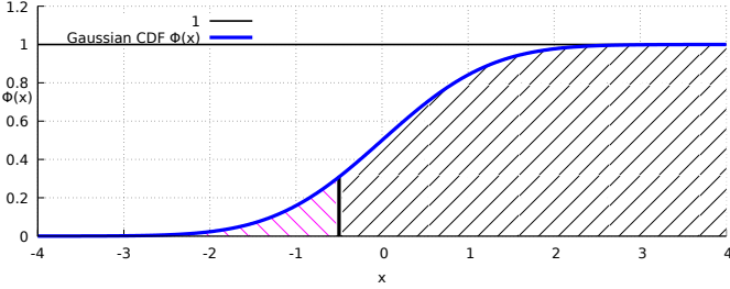
Fig. 1.12: Graph of the Gaussian Cumulative Distribution Function (CDF).
