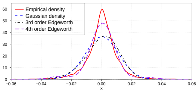
Fig. 1.23: Edgeworth expansions up to the fourth order.
