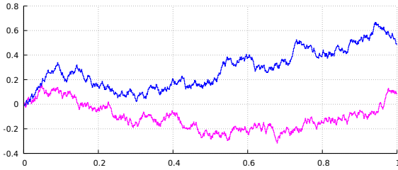
Fig. 1.3: Two sample paths of one-dimensional Brownian motion.
