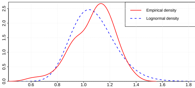
Fig. 1.21: Empirical density vs. normalized lognormal density.
