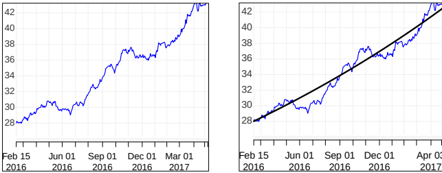
Fig. 1.15: Graph of simulated geometric Brownian motion.
