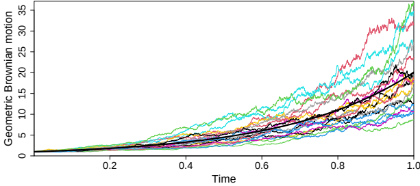
Fig. 1.11: Twenty sample paths of geometric Brownian motion (S_t)_{t \in \mathbb{R}_+} .
