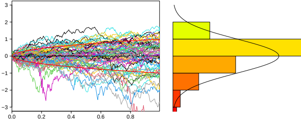
Fig. 1.16: Statistics of 72 yearly return graphs of the S&P 500 from 1950 to 2022.
