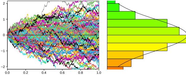
Fig. 1.6: Statistics of one-dimensional Brownian paths vs. Gaussian distribution.
