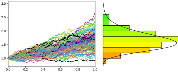
Fig. 1.13: Statistics of geometric Brownian paths vs. lognormal distribution.
