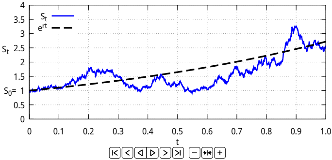
Fig. 1.10: Geometric Brownian motion started at S_0 = 1 , with \mu = r = 1 and \sigma^2 = 0.5 .*
