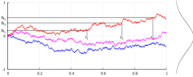
Fig. 1.7: Sample paths of a one-dimensional Brownian motion.
