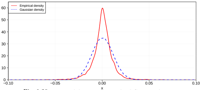
Fig. 1.20: Empirical density vs. normalized Gaussian density.
