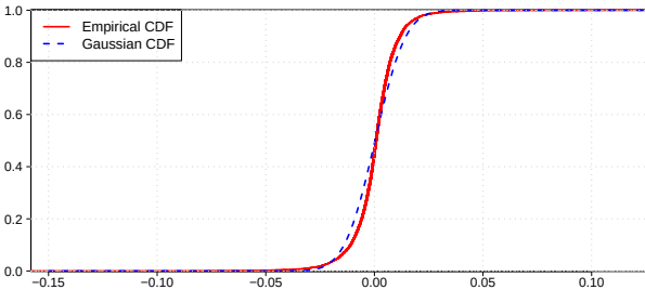
Fig. 1.18: Empirical vs. Gaussian CDF.
