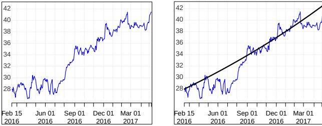
Fig. 1.14: HSBC Market price.
