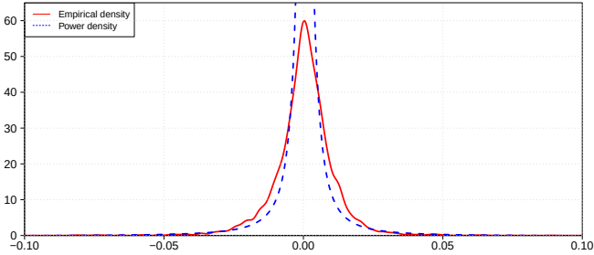
Fig. 1.22: Empirical density vs. power tail density.
