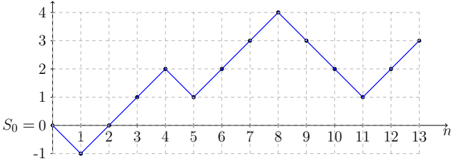
Fig. 1.1: Sample path of the random walk (S_n)_{n \geq 0} .
