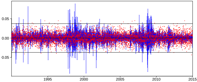
Fig. 1.17: Market returns (blue) vs. normalized Gaussian returns (red).
