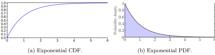
Fig. A.2: Exponential CDF and PDF.
