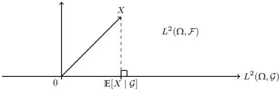
Fig. A.4: Conditional expectation as a projection.
