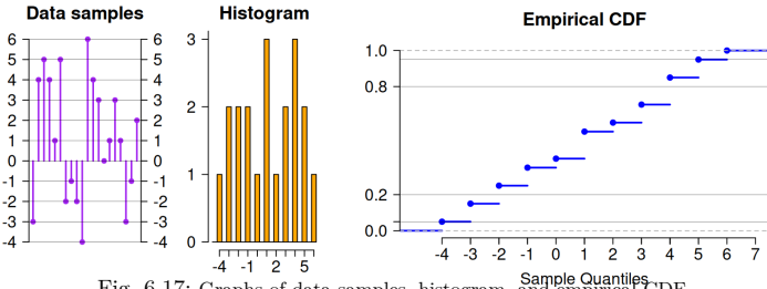
Fig. 6.17: Graphs of data samples, histogram, and empirical CDF.
