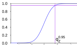
(a) Gaussian quantile q_Z^{0.95} and CDF.
