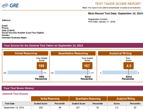
Fig. 6.6: Example of quantiles given as percentiles.
