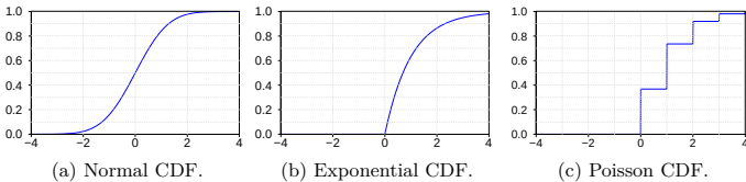
Fig. 6.3: Cumulative distribution functions.
