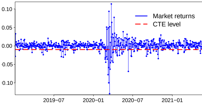
Fig. 6.1: Estimating liabilities by the conditional mean \mathbb{E}[X \mid X < 0] .
