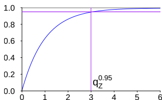
(a) Exponential quantile q_Z^{0.95} and CDF.
