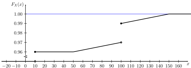
Fig. 6.16: Cumulative distribution function of X .
