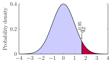
(b) Gaussian quantile q_Z^{0.95} and PDF.
