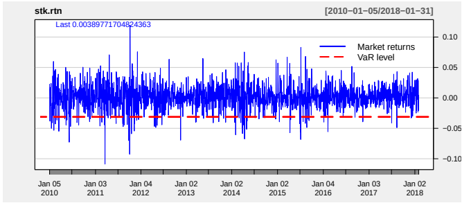
Fig. 6.15: Market returns vs. Value at Risk level in red.
