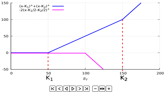
Fig. S.27: Butterfly option as a combination of call options.*
