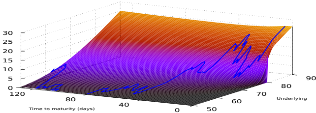
Fig. S.61: Price map of the European knock-in call option.
