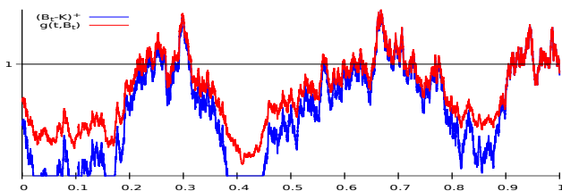
Fig. S.18: Risk-neutral pricing of the FX option by \pi_t(B_t) = g(t, B_t) vs stop-loss/start-gain pricing.
