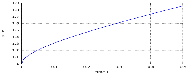
Fig. S.67: Expected maximum of geometric Brownian motion over [0, T] .
