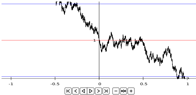
Fig. S.16: Brownian crossings of level 1.*
