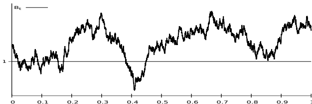
Fig. S.17: Brownian path started at B_0 > 1 .
