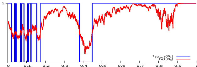
Fig. S.19: Delta hedging of the FX option by \xi_t = h(t, B_t) vs the stop-loss/start-gain strategy.
