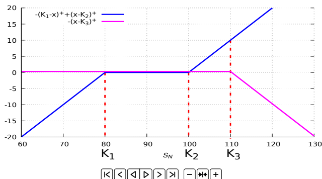
Fig. S.10: Call spread collar payoff as a combination of call and put option payoffs.*
