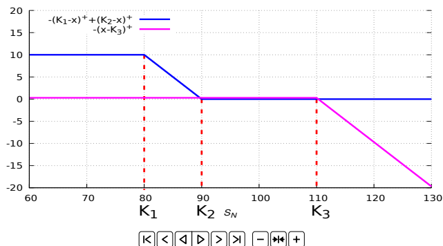
Fig. S.7: Put spread collar payoff as a combination of call and put option payoffs.*
