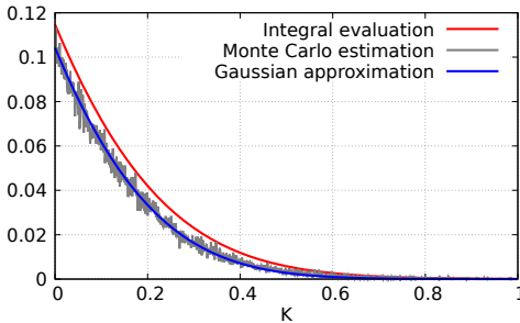
Fig. S.30: Gaussian approximation of spread option prices.
