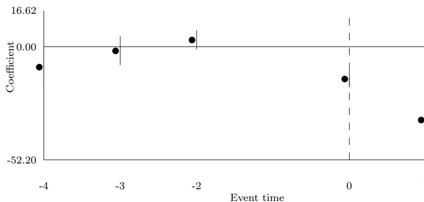
Figure 1: NOMIS Claimant Count event-study profile
