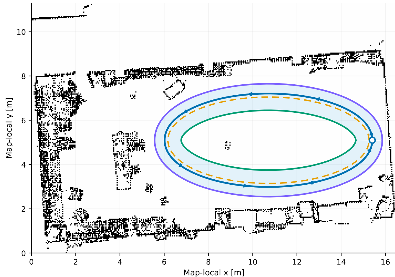
Virtual Race Track Generated from the Point-LIO Occupancy Map Full Point-LIO Map with Virtual Track
