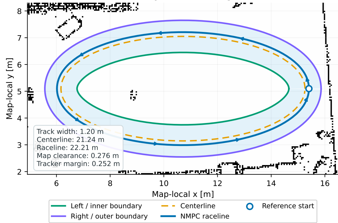
Track Geometry and Tracking Reference
