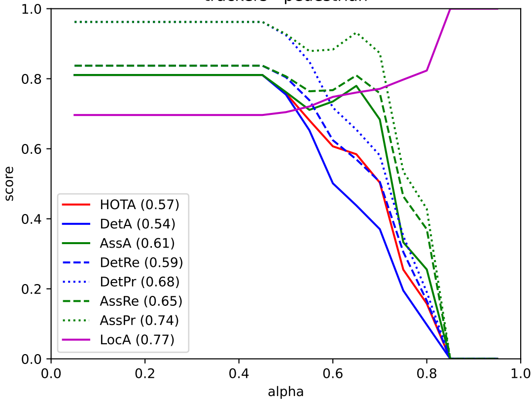
trackers - pedestrian
