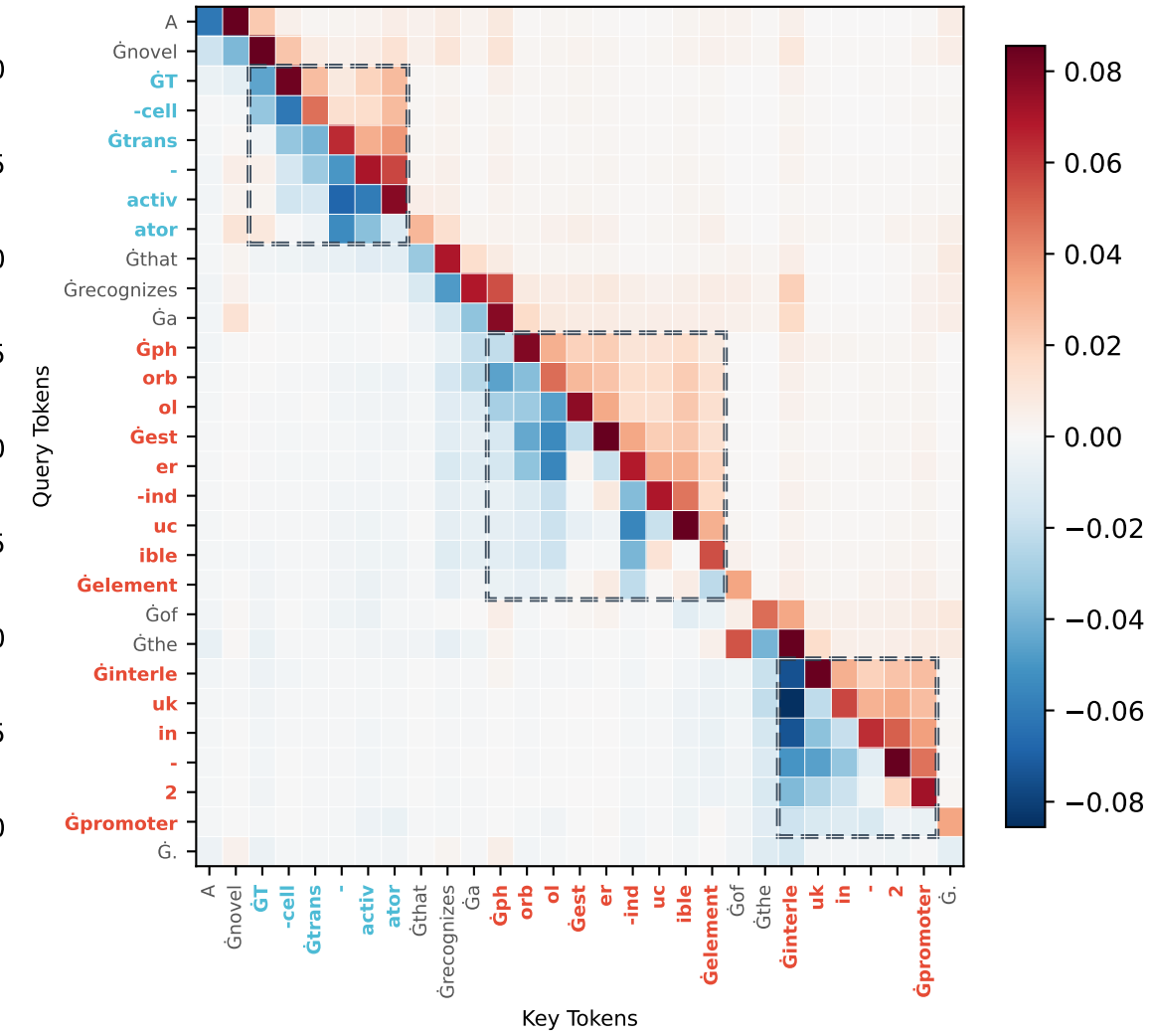
(f) \Delta Attention (D – C)
