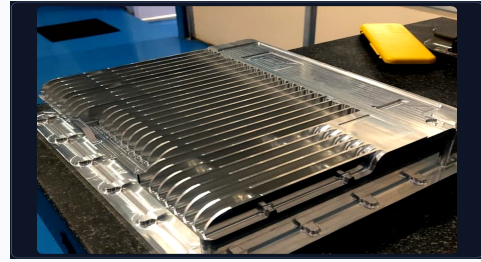
Finned Cold Plate (Thin Fin) High-Aspect Ratio Heat Sink • Electronics
