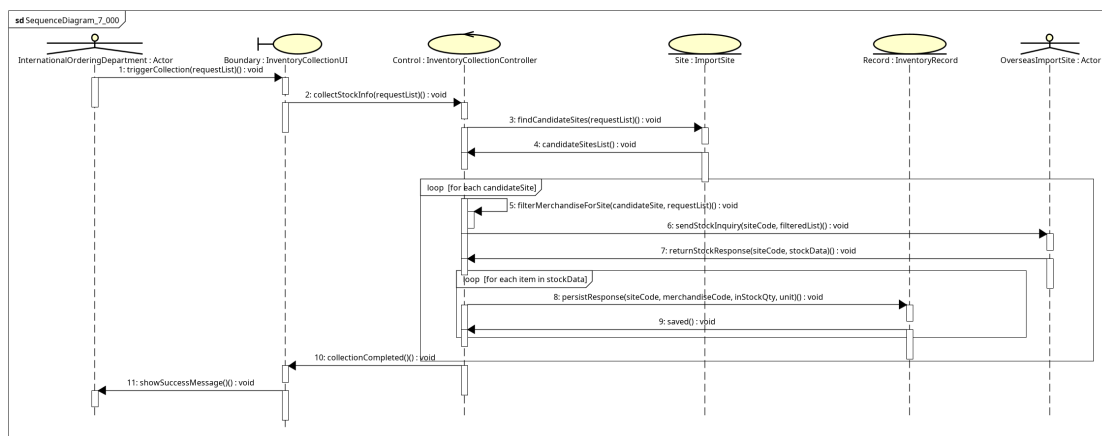
Figure 3.1: Sequence diagram mức phân tích UC003 - CollectInventory-Data
