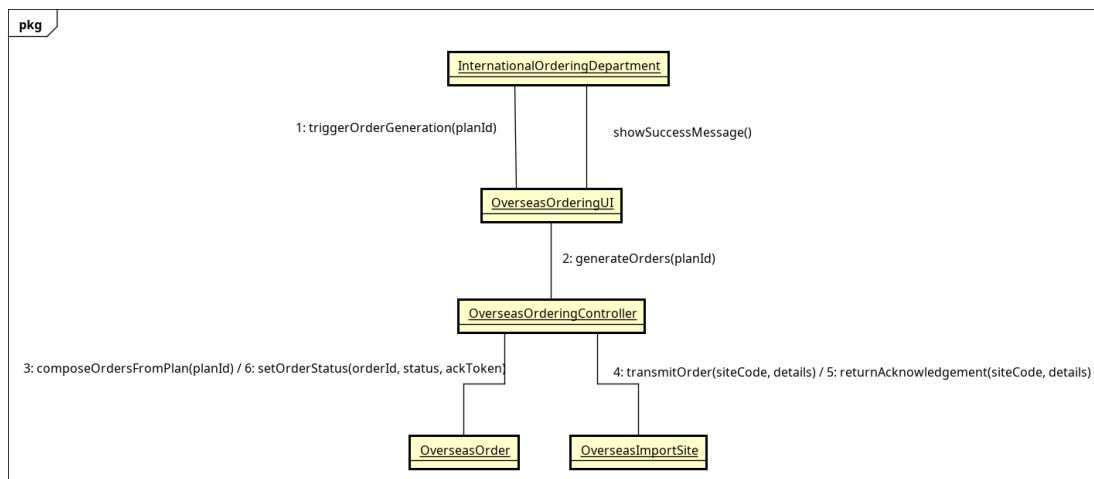
Figure 3.15: Communication diagram mức phân tích UC005 - PlaceOverseasOrders
