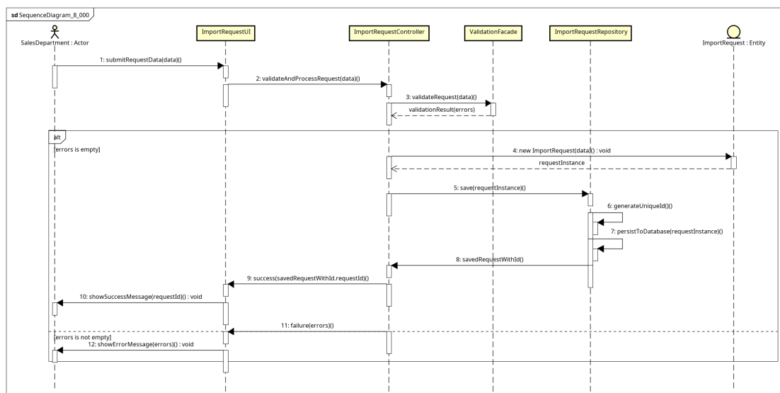
Figure 3.1: Sequence diagram mức thiết kế UC001 - ManageImportRequests
