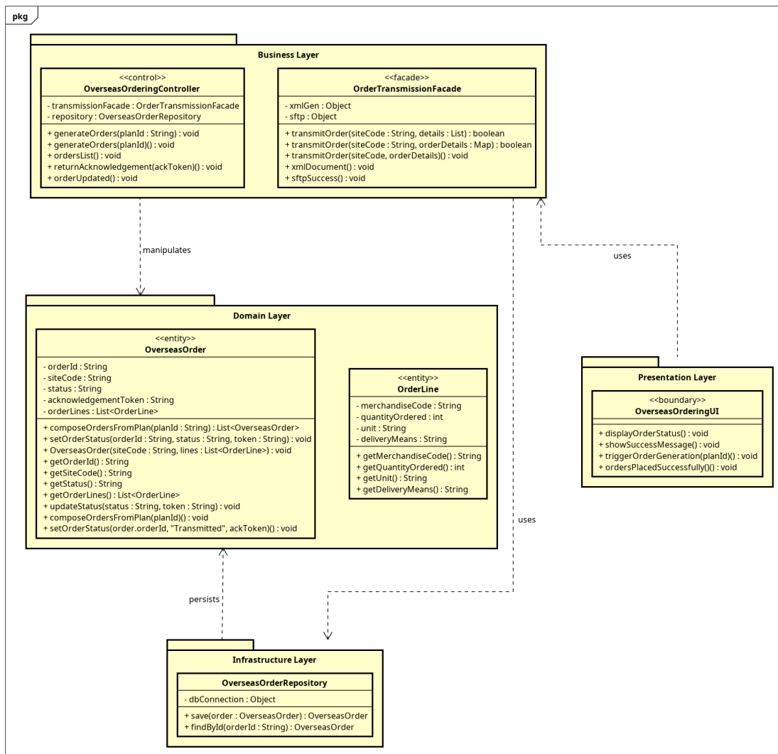
Figure 3.2: Package dependency diagram UC005 - PlaceOverseasOrders
