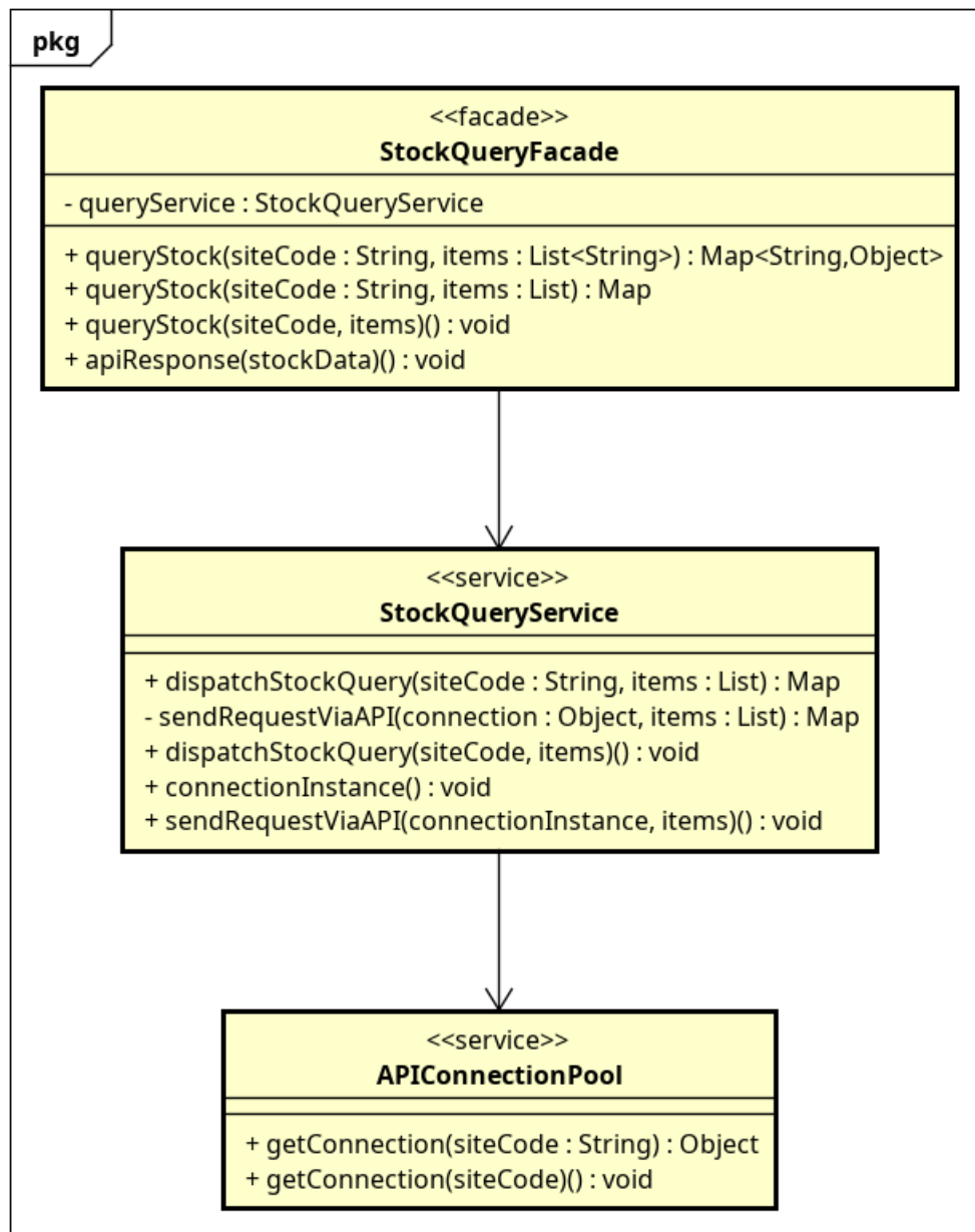
Figure 3.3: Class diagram subsystem UC003 - CollectInventoryData
