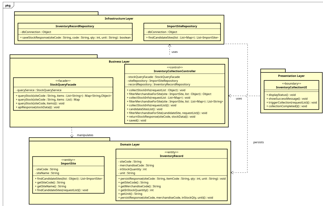
Figure 3.2: Package dependency diagram UC03 - CollectInventoryData
