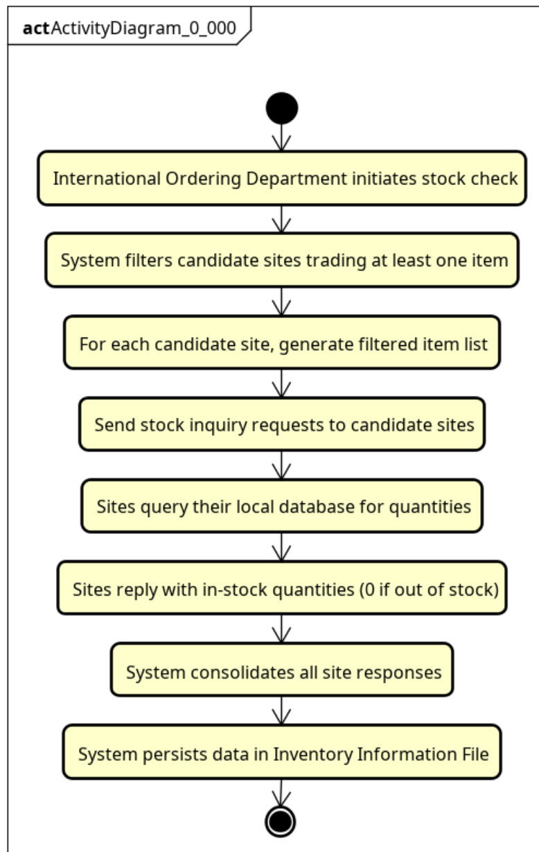
Figure 3.2: Activity diagram UC003 - CollectInventoryData
