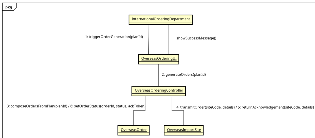
Figure 3.2: Communication diagram mức phân tích UC005 - PlaceOverseasOrders
