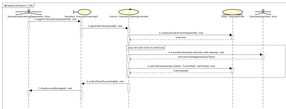
Figure 3.1: Sequence diagram mức phân tích UC005 - PlaceOverseasOrders
