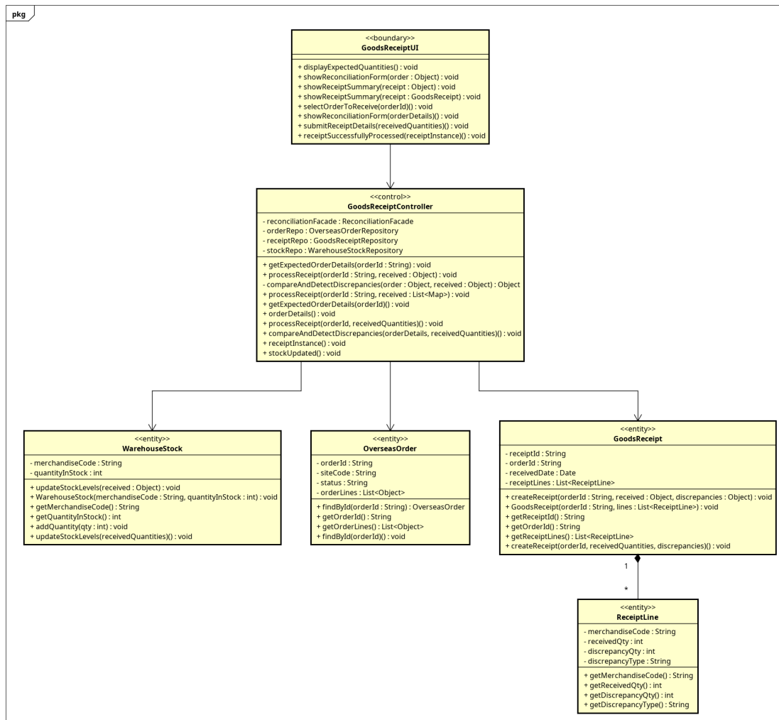
Figure 3.3: Class diagram mức phân tích UC006 - ReceiveAndReconcile-Goods
