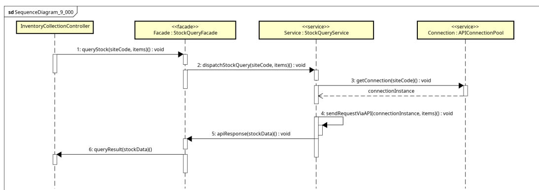
Figure 3.3: Sequence diagram subsystem UC003 - CollectInventoryData
