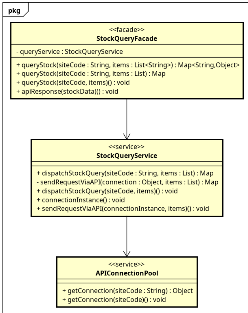
Figure 3.2: Class diagram subsystem UC003 - CollectInventoryData
