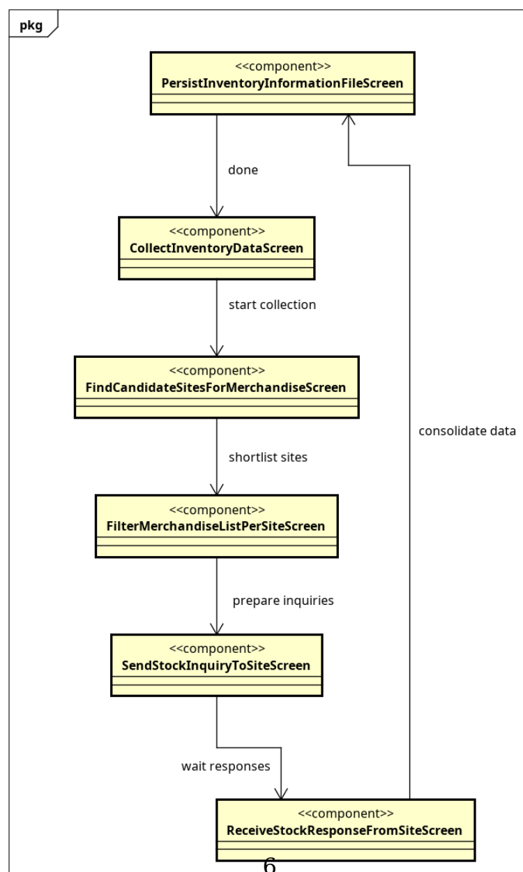
Figure 3.1: Screen transition diagram UC003 - CollectInventoryData
