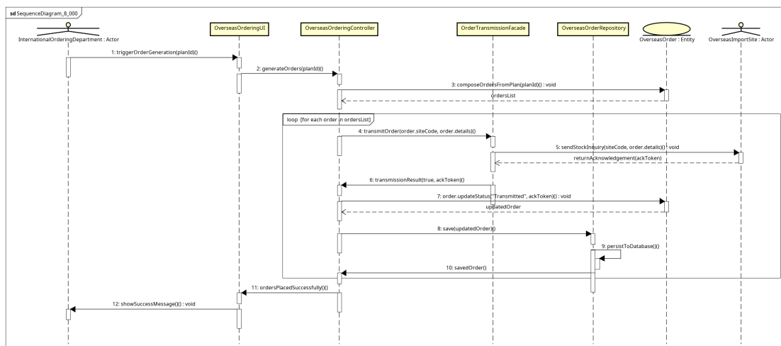
Figure 3.1: Sequence diagram mức thiết kế UC005 - PlaceOverseasOrders
