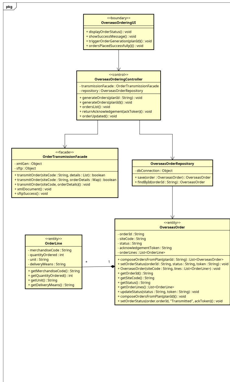
Figure 3.2: Class diagram mức thiết kế UC005 - PlaceOverseasOrders
