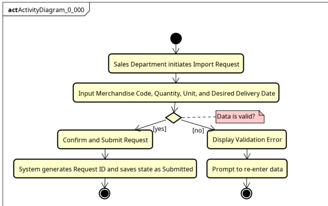
Figure 3.2: Activity diagram UC001 - ManageImportRequests
