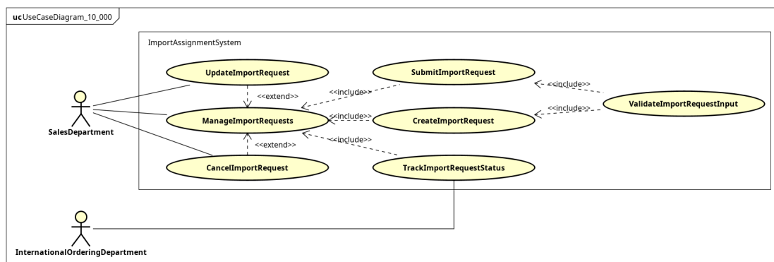
Figure 3.1: Use case phân rã UC001 - ManageImportRequests
