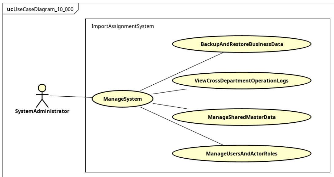
Figure 3.3: Use case phân rã UC007 - ManageSystem
