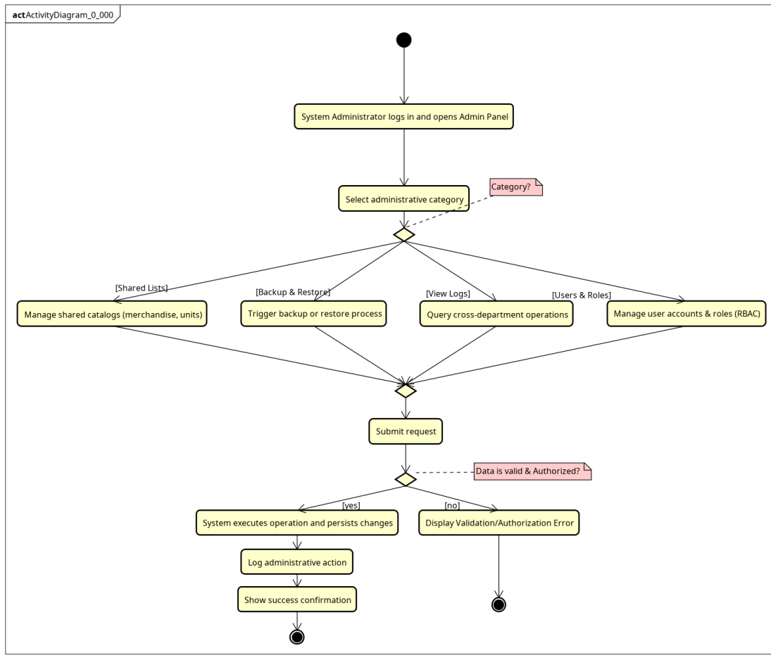
Figure 3.4: Activity diagram UC007 - ManageSystem
