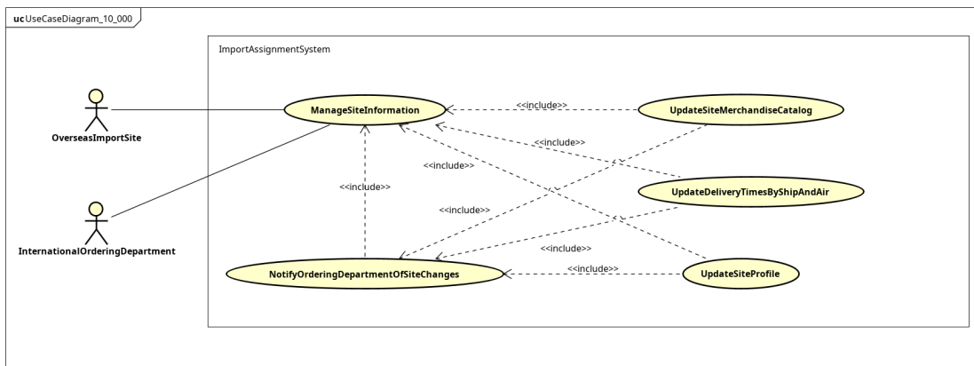
Figure 3.1: Use case phân rã UC002 - ManageSiteInformation
