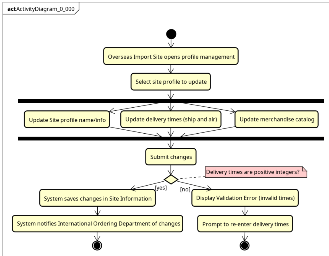
Figure 3.2: Activity diagram UC002 - ManageSiteInformation
