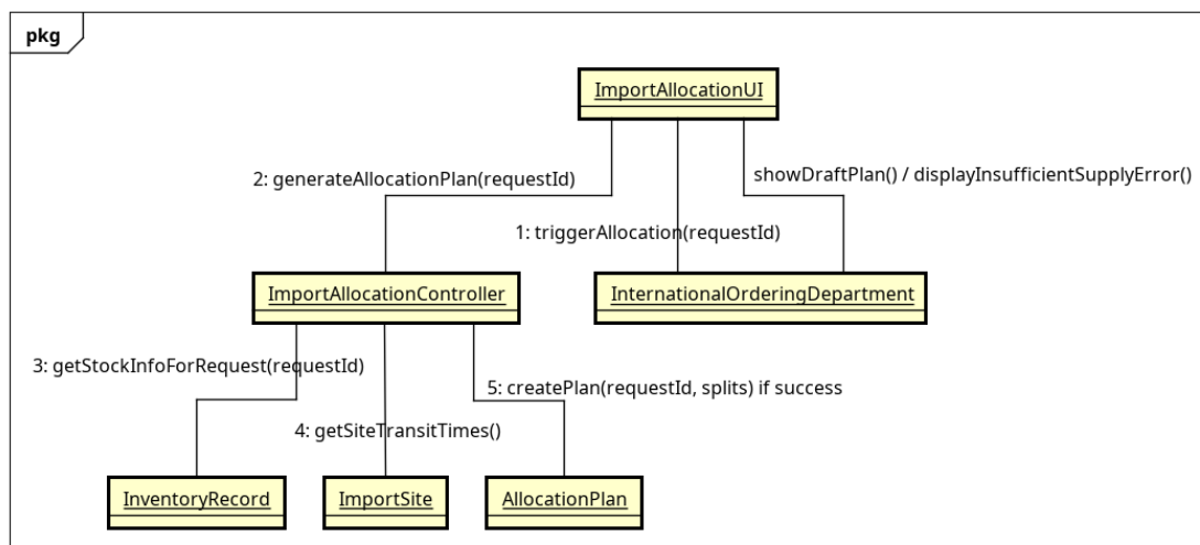
Figure 3.12: Communication diagram mức phân tích UC004 - PlanImportAllocation
