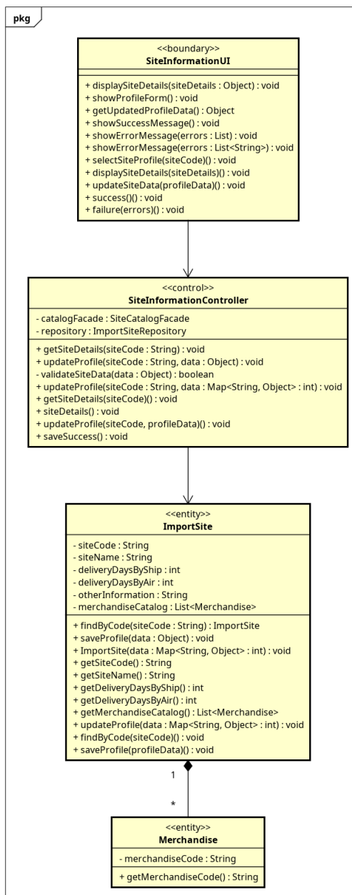
Figure 3.7: Class diagram mức phân tích UC002 - ManageSiteInformation
