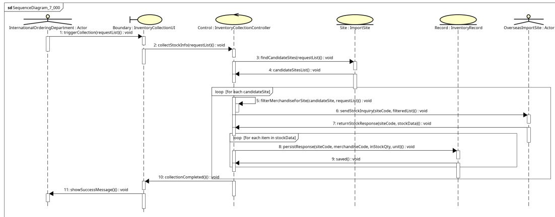
Figure 3.8: Sequence diagram mức phân tích UC003 - CollectInventory-Data
