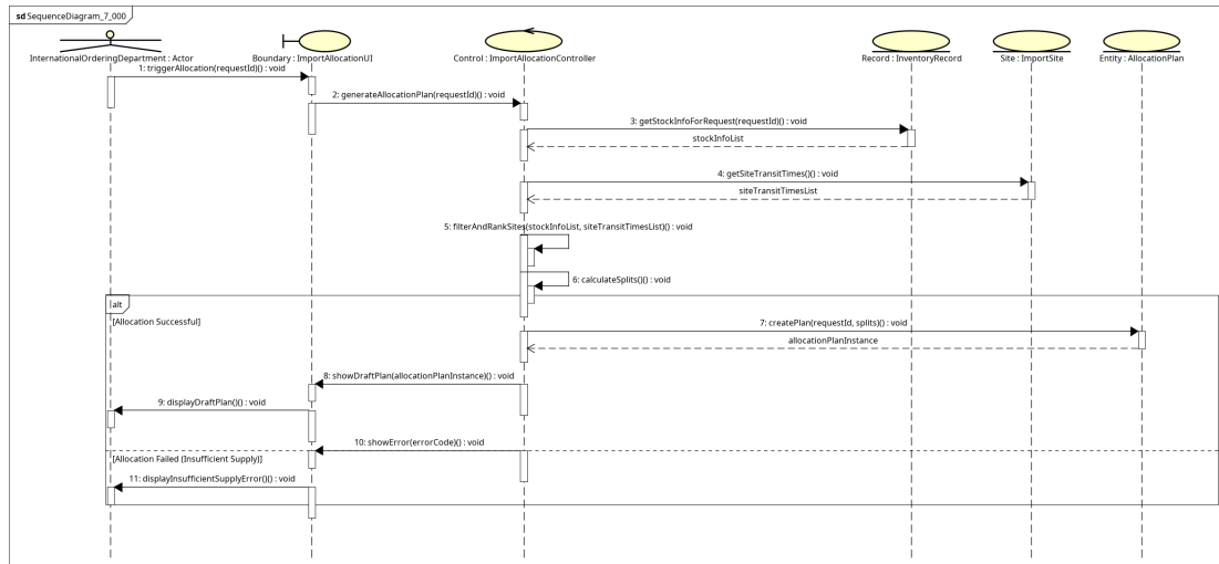
Figure 3.11: Sequence diagram mức phân tích UC004 - PlanImportAllocation
