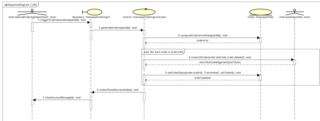
Figure 3.14: Sequence diagram mức phân tích UC005 - PlaceOverseasOrders
