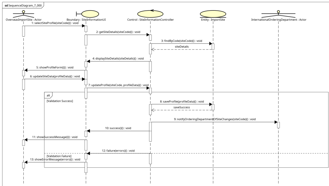
Figure 3.5: Sequence diagram mức phân tích UC002 - ManageSiteInformation
