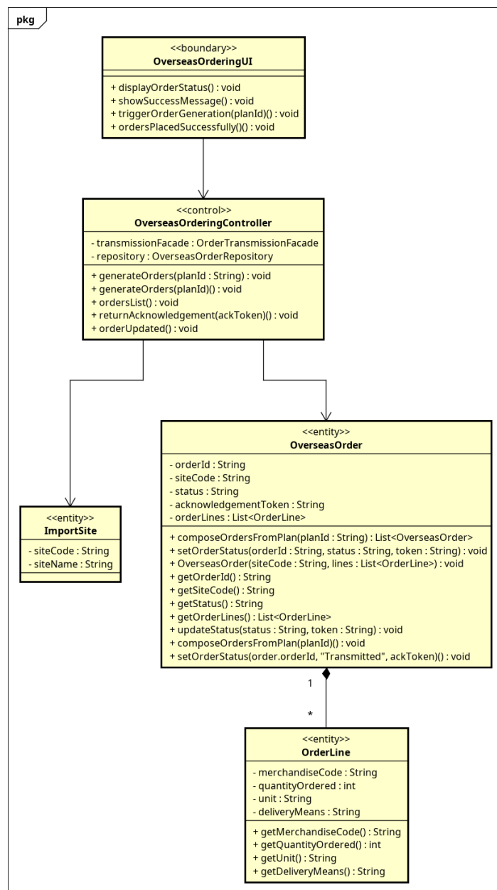
Figure 3.16: Class diagram mức phân tích UC005 - PlaceOverseasOrders
