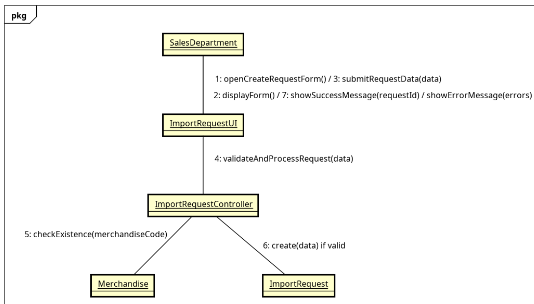
Figure 3.3: Communication diagram mức phân tích UC001 - ManageImportRequests
