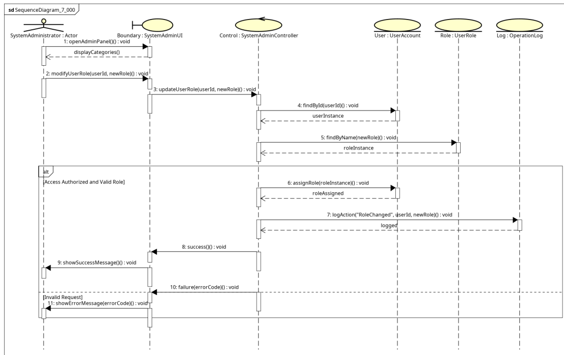
Figure 3.20: Sequence diagram mức phân tích UC007 - ManageSystem
