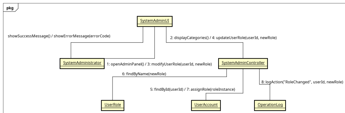
Figure 3.21: Communication diagram mức phân tích UC007 - ManageSystem
