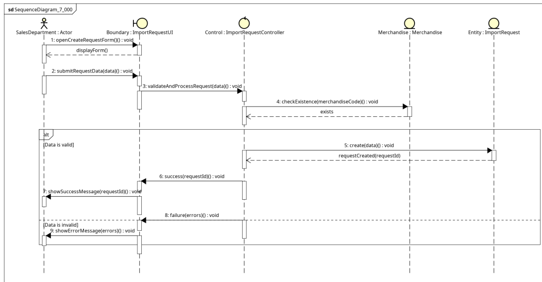
Figure 3.2: Sequence diagram mức phân tích UC001 - ManageImportRequests
