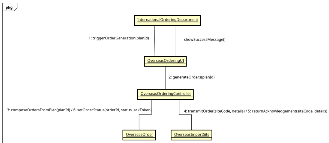
Figure 3.15: Communication diagram mức phân tích UC005 - PlaceOverseasOrders
