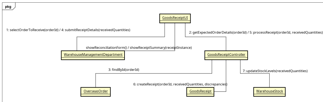
Figure 3.18: Communication diagram mức phân tích UC006 - Receive-AndReconcileGoods
