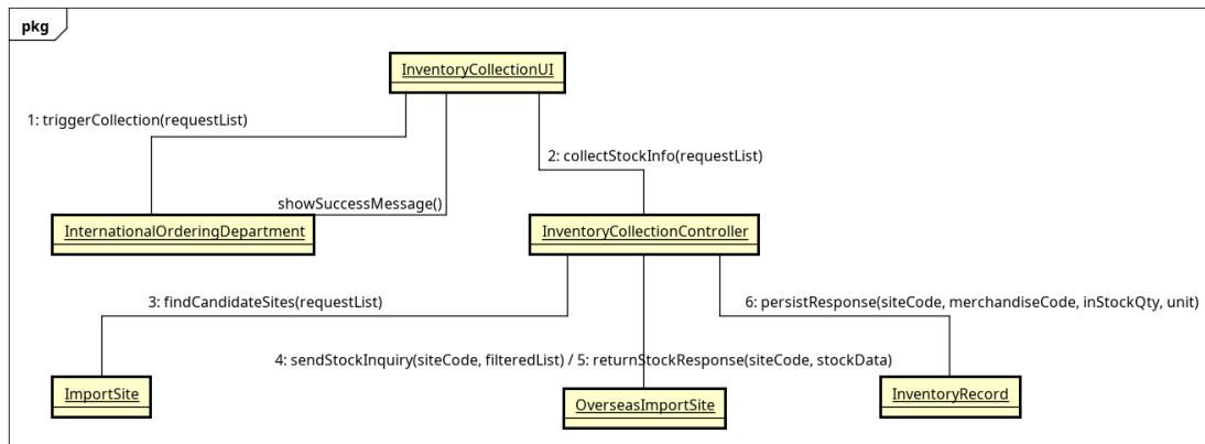
Figure 3.9: Communication diagram mức phân tích UC003 - CollectInventoryData
