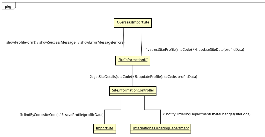
Figure 3.6: Communication diagram mức phân tích UC002 - ManageSiteInformation
