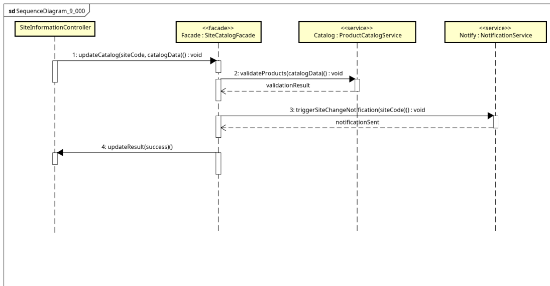
Figure 3.3: Sequence diagram subsystem UC002 - ManageSiteInformation
