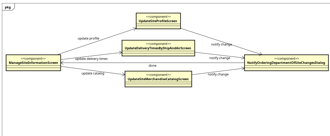
Figure 3.1: Screen transition diagram UC002 - ManageSiteInformation
