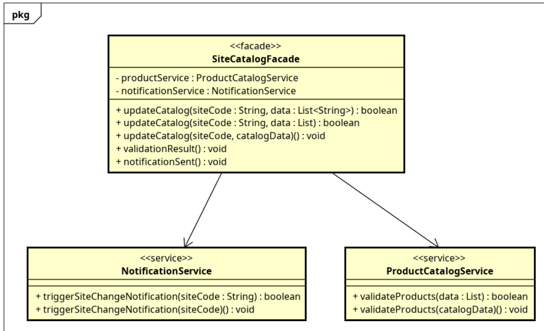
Figure 3.2: Class diagram subsystem UC002 - ManageSiteInformation
