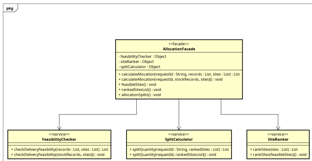
Figure 3.2: Class diagram subsystem UC004 - PlanImportAllocation
