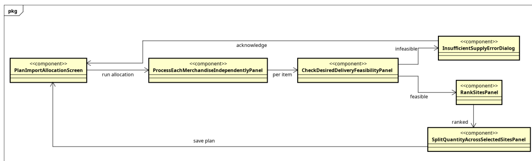
Figure 3.1: Screen transition diagram UC004 - PlanImportAllocation
