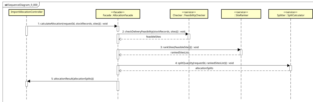
Figure 3.3: Sequence diagram subsystem UC004 - PlanImportAllocation
