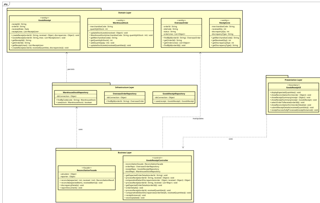
Figure 3.3: Package dependency diagram UC006 - ReceiveAndReconcileGoods
