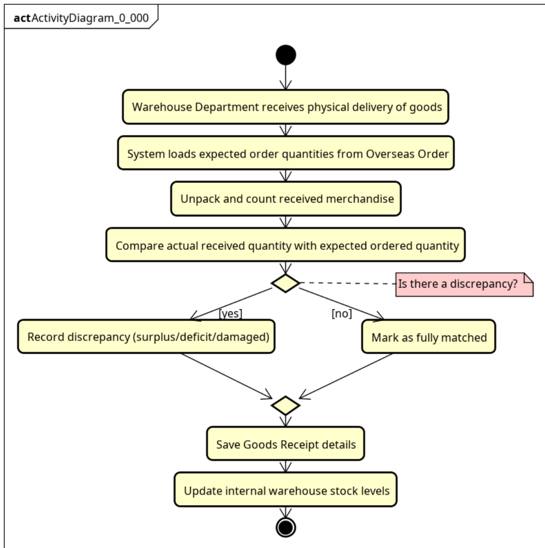
Figure 3.2: Activity diagram UC006 - ReceiveAndReconcileGoods
