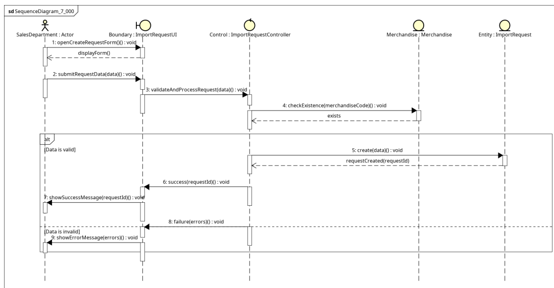
Figure 3.1: Sequence diagram mức phân tích UC001 - ManageImportRequests
