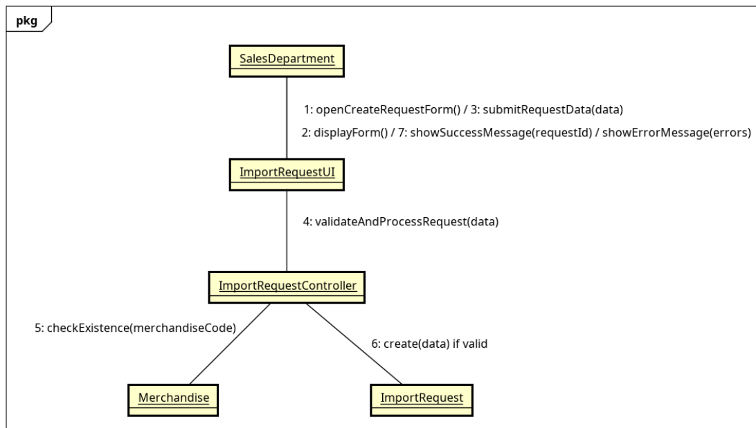
Figure 3.2: Communication diagram mức phân tích UC001 - ManageImportRequests
