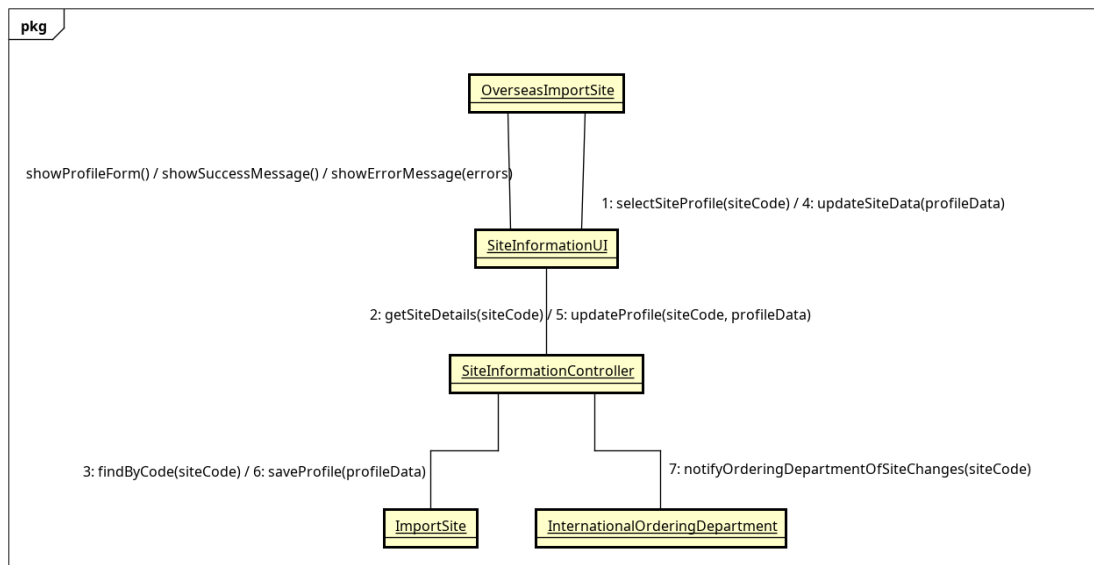
Figure 3.2: Communication diagram mức phân tích UC002 - ManageSite-Information
