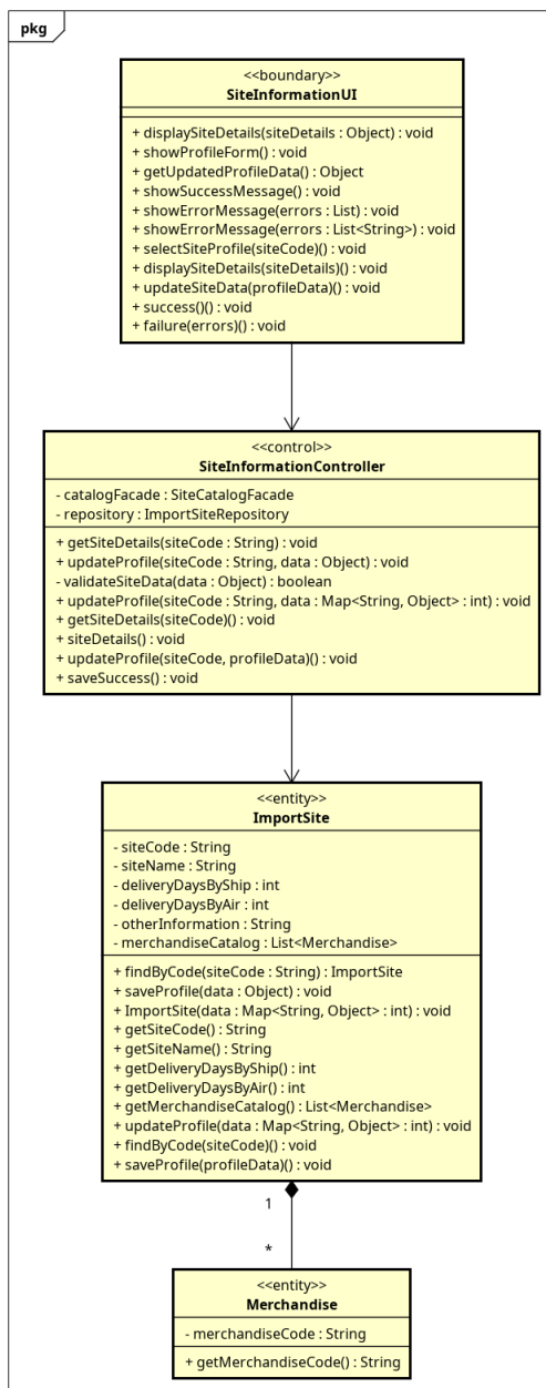
Figure 3.3: Class diagram mức phân tích UC002 - ManageSiteInformation
