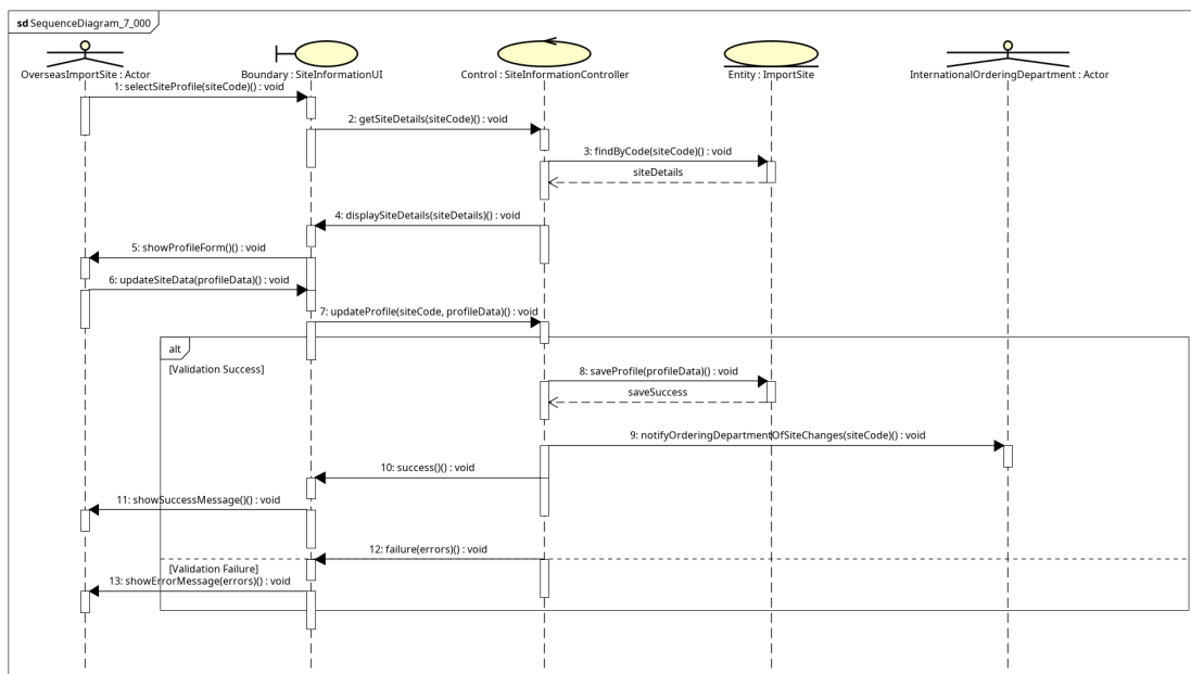
Figure 3.1: Sequence diagram mức phân tích UC002 - ManageSiteInformation
