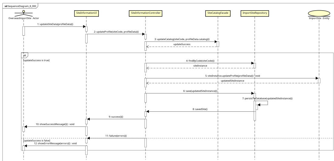
Figure 3.1: Sequence diagram mức thiết kế UC002 - ManageSiteInformation
