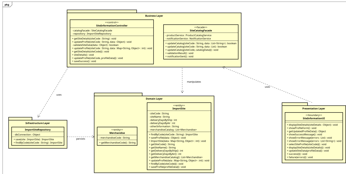
Figure 3.3: Package dependency diagram UC002 - ManageSiteInformation
