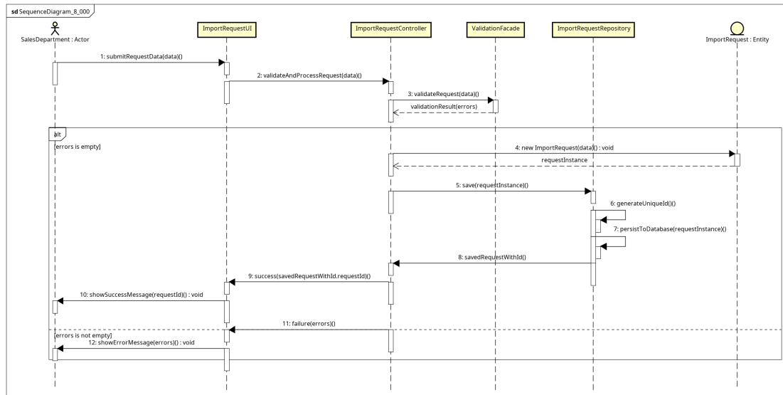
Figure 3.2: Sequence diagram mức thiết kế UC001 - ManageImportRequests
