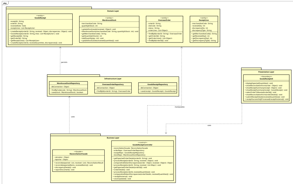
Figure 3.19: Package dependency diagram UC006 - ReceiveAndReconcileGoods
