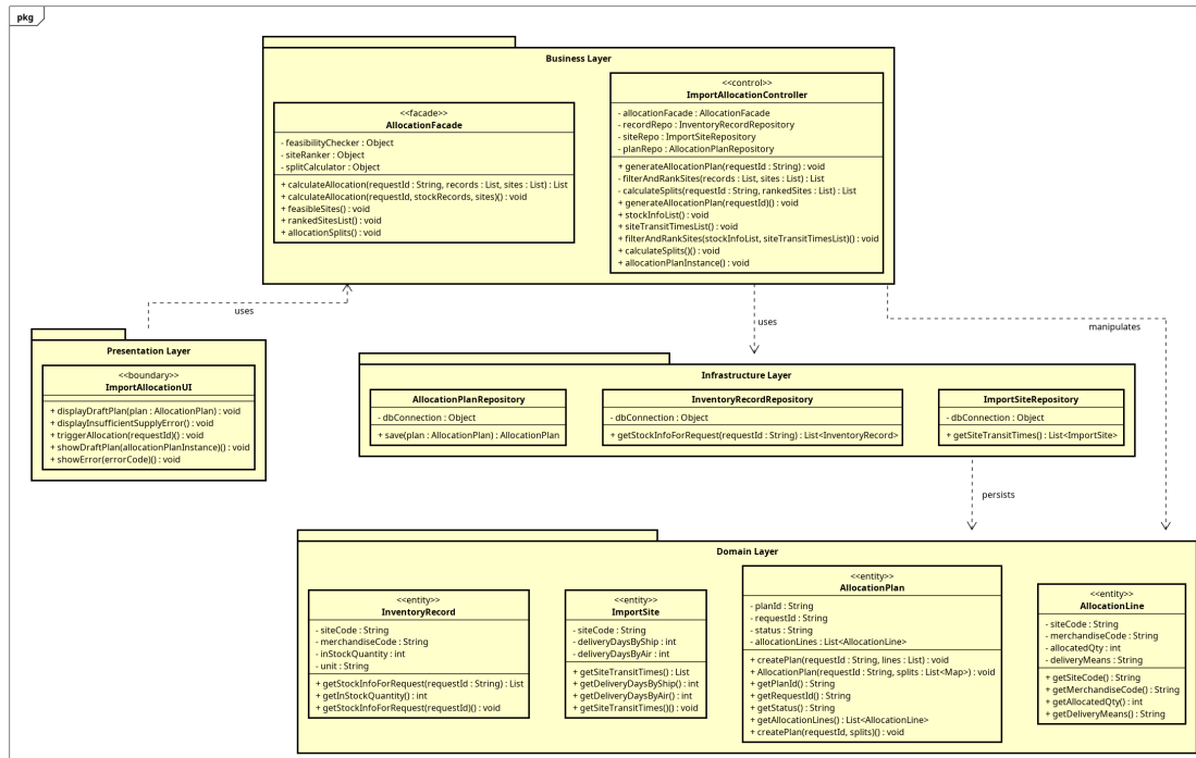
Figure 3.13: Package dependency diagram UC004 - PlanImportAllocation
