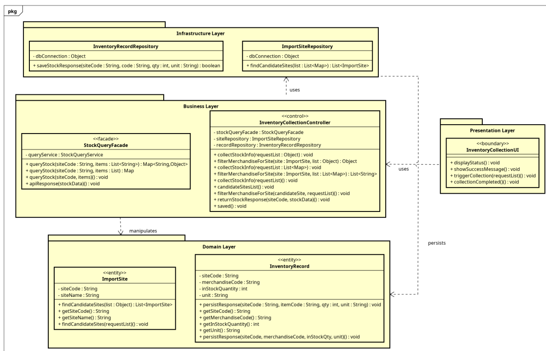
Figure 3.10: Package dependency diagram UC003 - CollectInventory-Data
