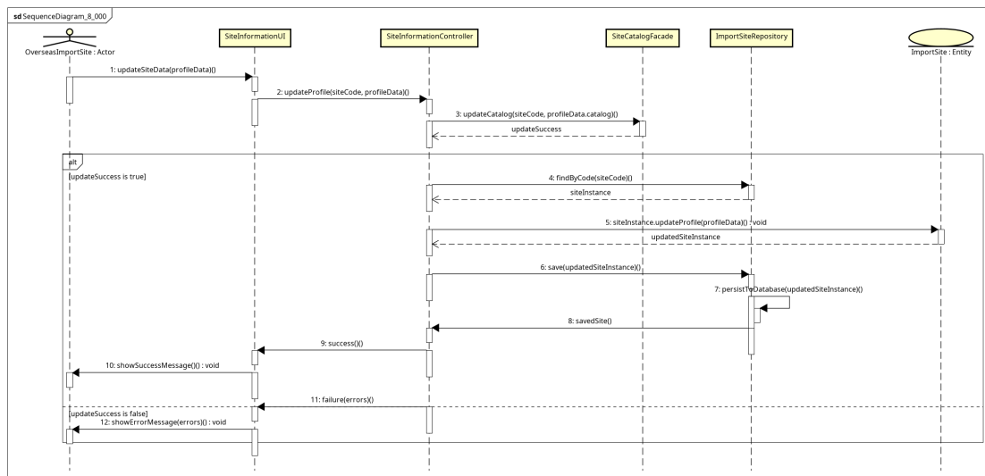
Figure 3.5: Sequence diagram mức thiết kế UC002 - ManageSiteInformation
