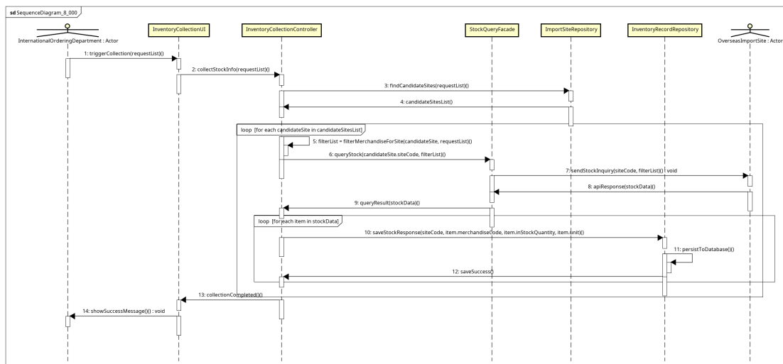
Figure 3.8: Sequence diagram mức thiết kế UC003 - CollectInventory-Data
