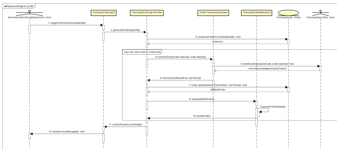
Figure 3.14: Sequence diagram mức thiết kế UC005 - PlaceOverseasOrders
