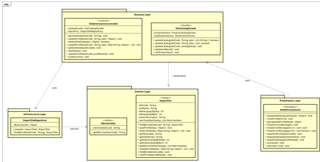
Figure 3.7: Package dependency diagram UC002 - ManageSiteInformation
