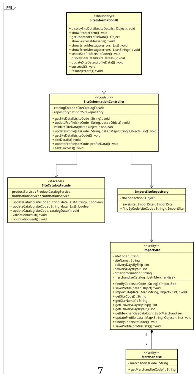
Figure 3.1: Class diagram mức thiết kế UC002 - ManageSiteInformation
