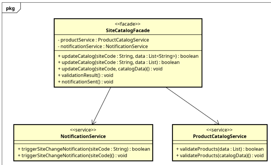
Figure 3.3: Class diagram subsystem UC002 - ManageSiteInformation
