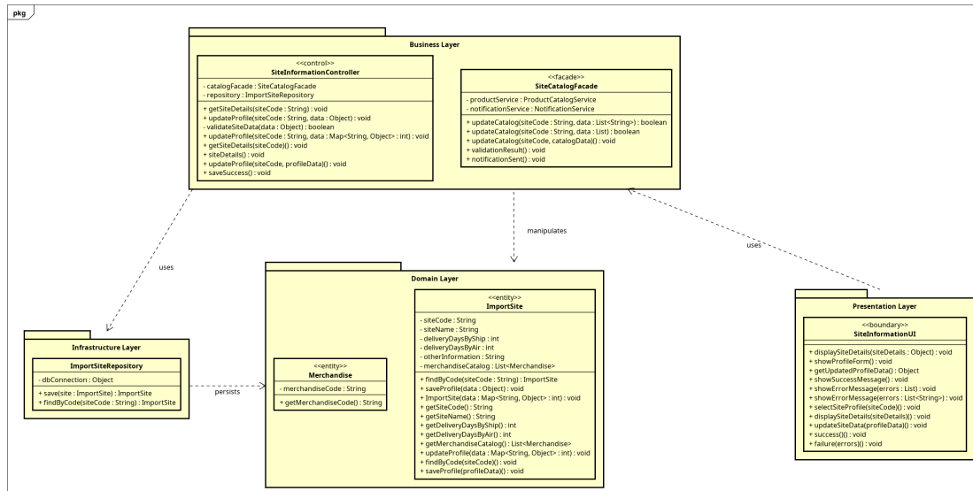
Figure 3.2: Package dependency diagram UC002 - ManageSiteInformation
