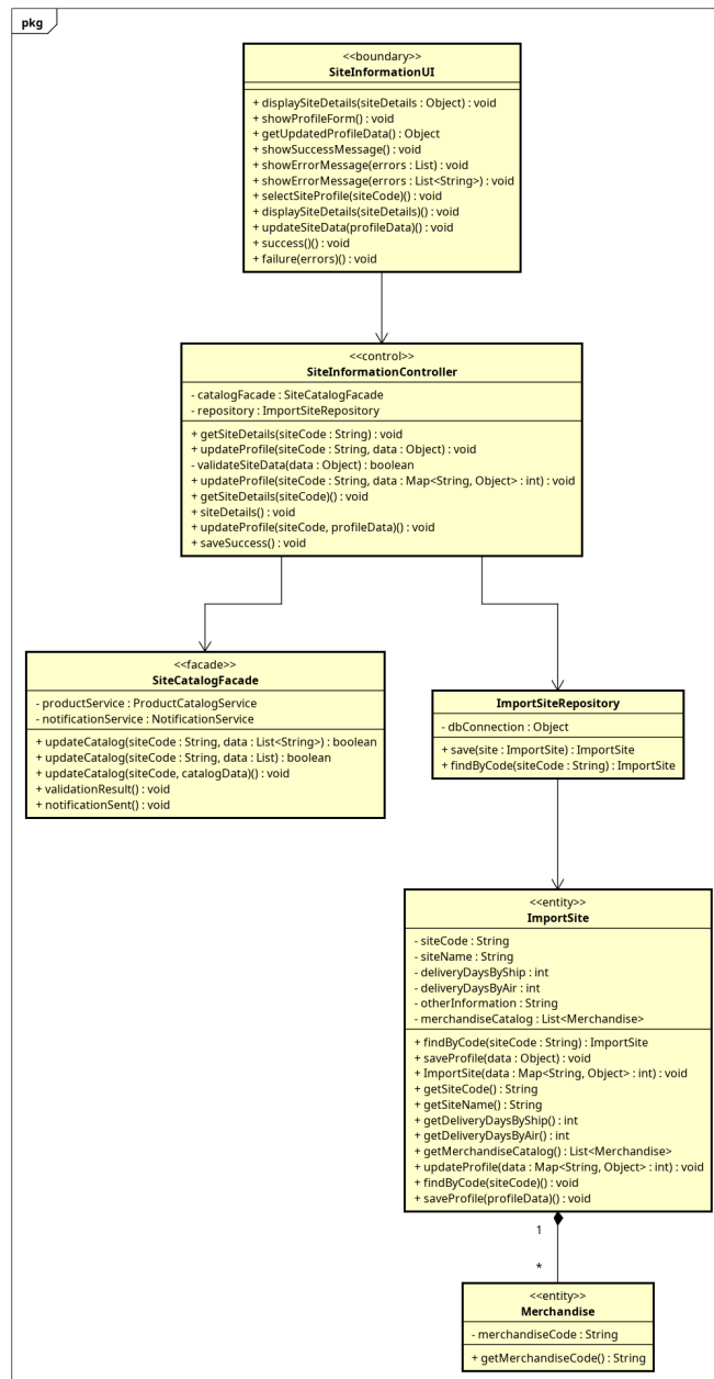
Figure 3.5: Class diagram mức thiết kế UC002 - ManageSiteInformation
