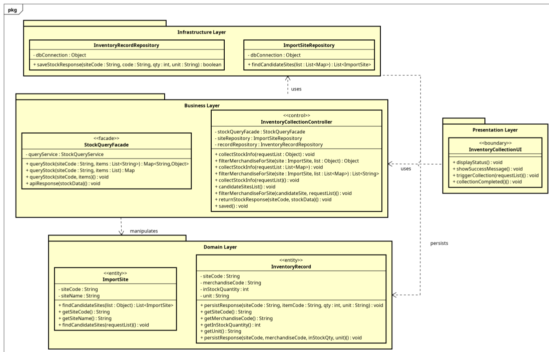
Figure 3.9: Package dependency diagram UC003 - CollectInventoryData
