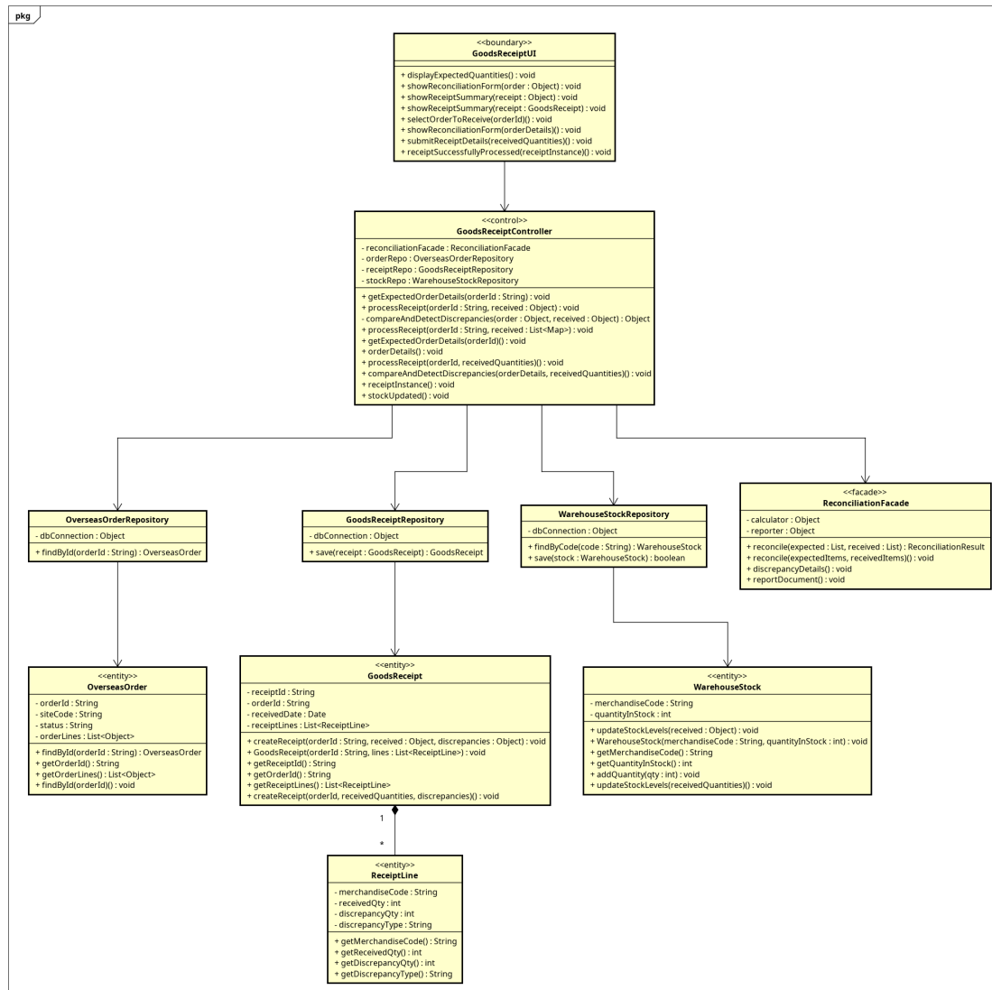
Figure 3.17: Class diagram mức thiết kế UC006 - ReceiveAndReconcile-Goods
