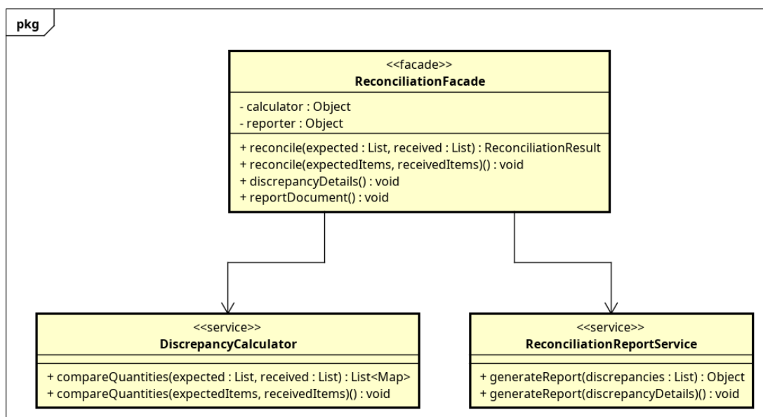
Figure 3.19: Class diagram subsystem UC006 - ReceiveAndReconcileGoods
