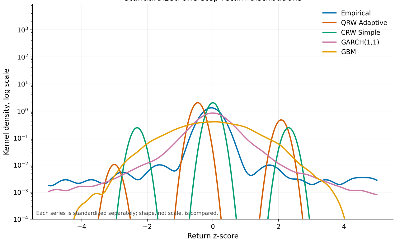
Standardized one-step return distributions
