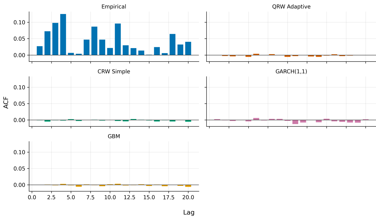
One-step return autocorrelation
