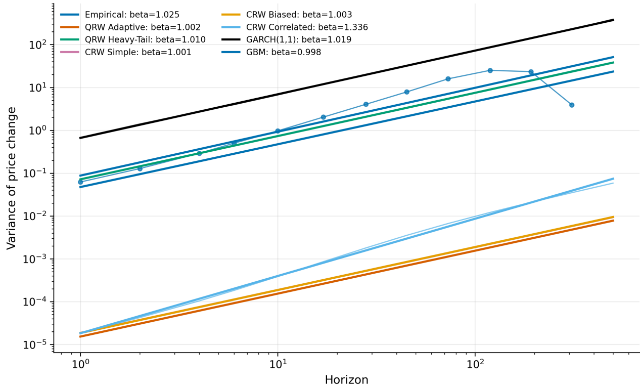
Variance scaling across empirical and simulated paths
