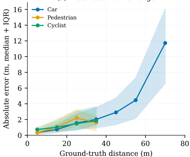
(a) Distance error vs. range
