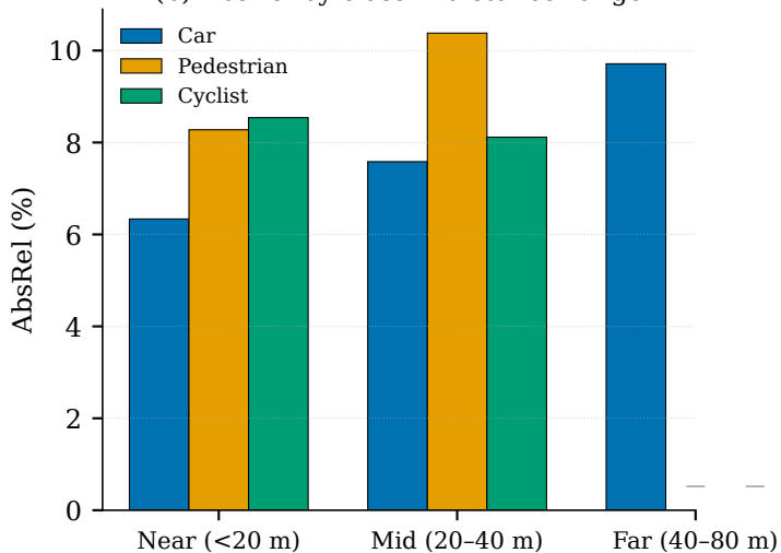
(b) AbsRel by class \times distance range
