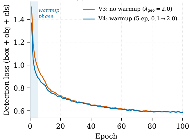
(a) Detection loss
