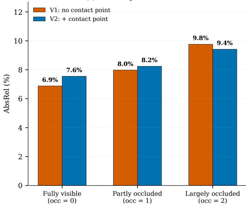
(a) AbsRel by occlusion level
