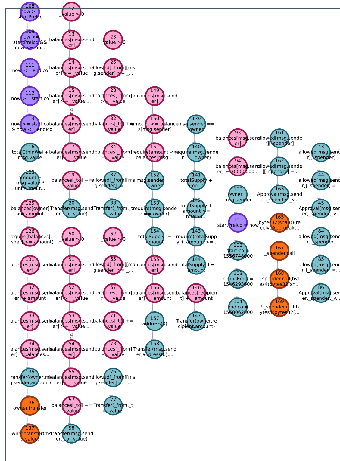
Denoised CFG 84 key nodes, 52 edges
