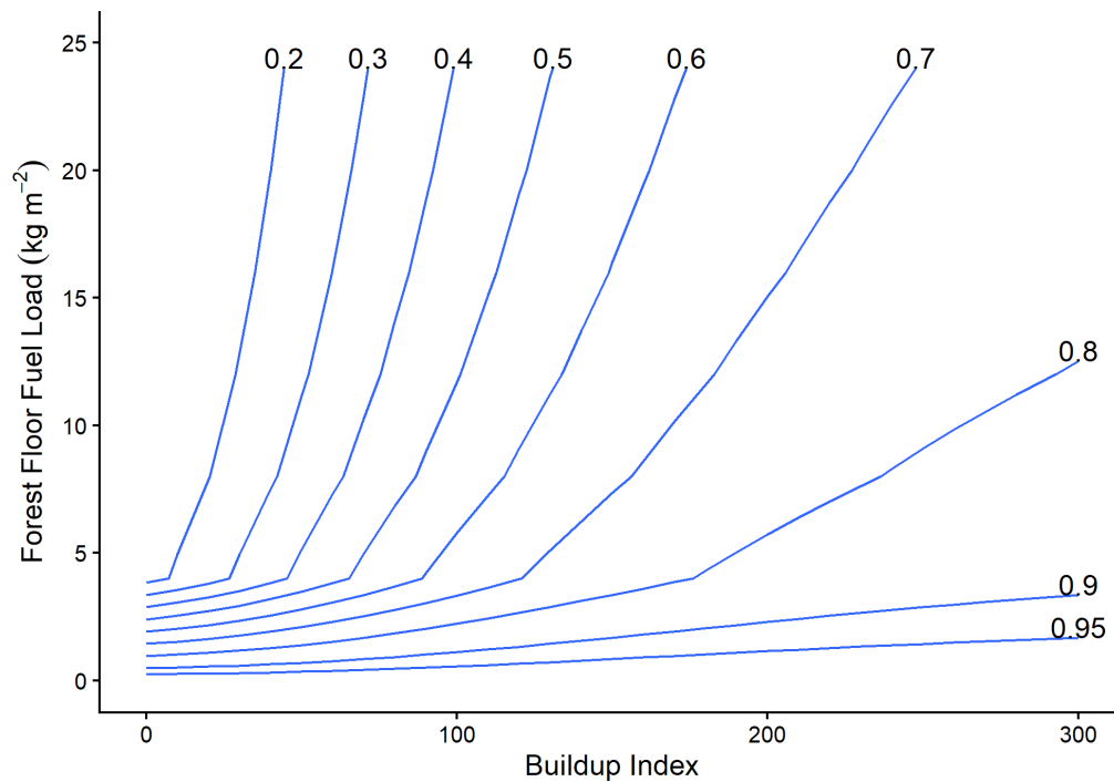
Figure C4. Isoline contours of equal organic soil layer consumption fraction as a function of BUI and the organic soil layer Carbon pool in kg/m 2 . Field observations of burn from 547 field measurements across Canada from the Yukon-Alaska border to Manitoba.
