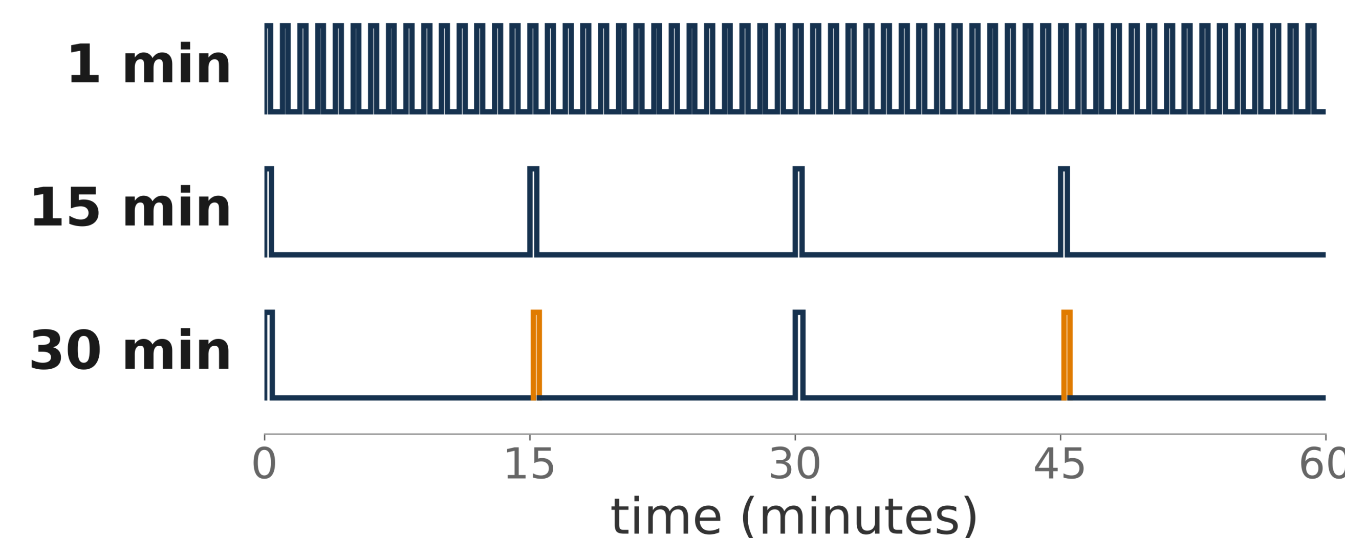
Figure 3: Radio duty cycle over one hour at each reporting rate (dark pulses are uploads, orange are keepalive pings)
