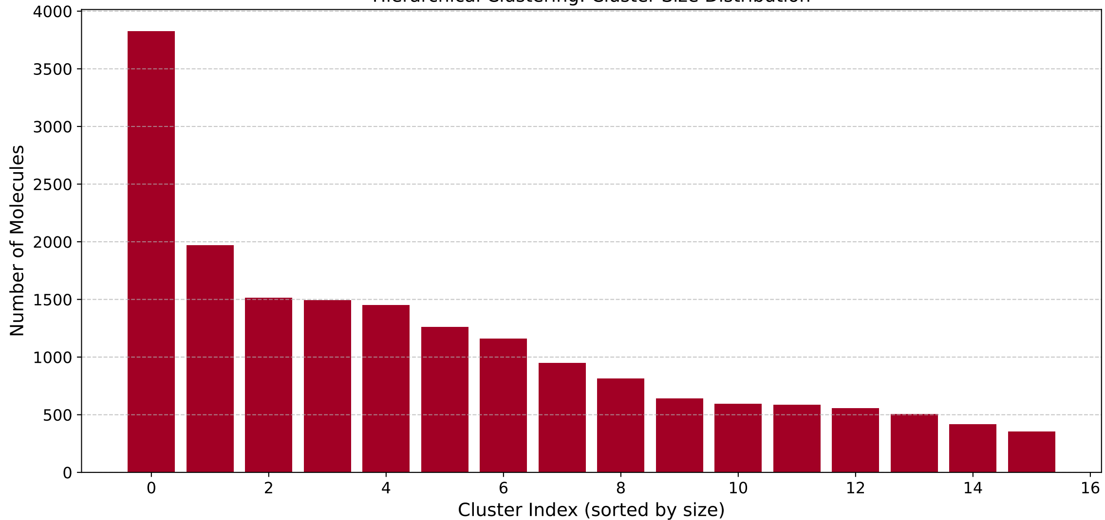
Hierarchical Clustering: Cluster Size Distribution
