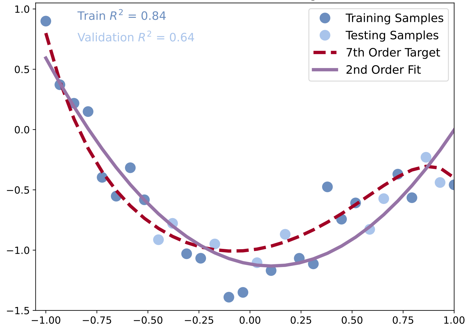
2nd Order Model Underfits: High Bias
