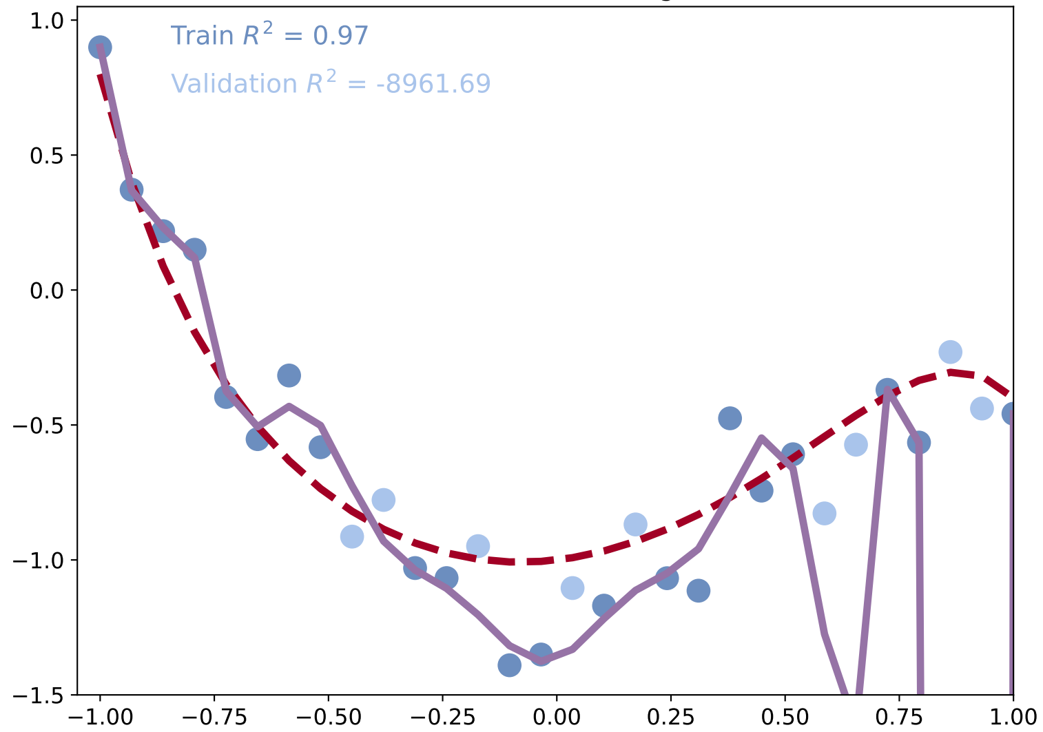
20th Order Model Overfits: High Variance
