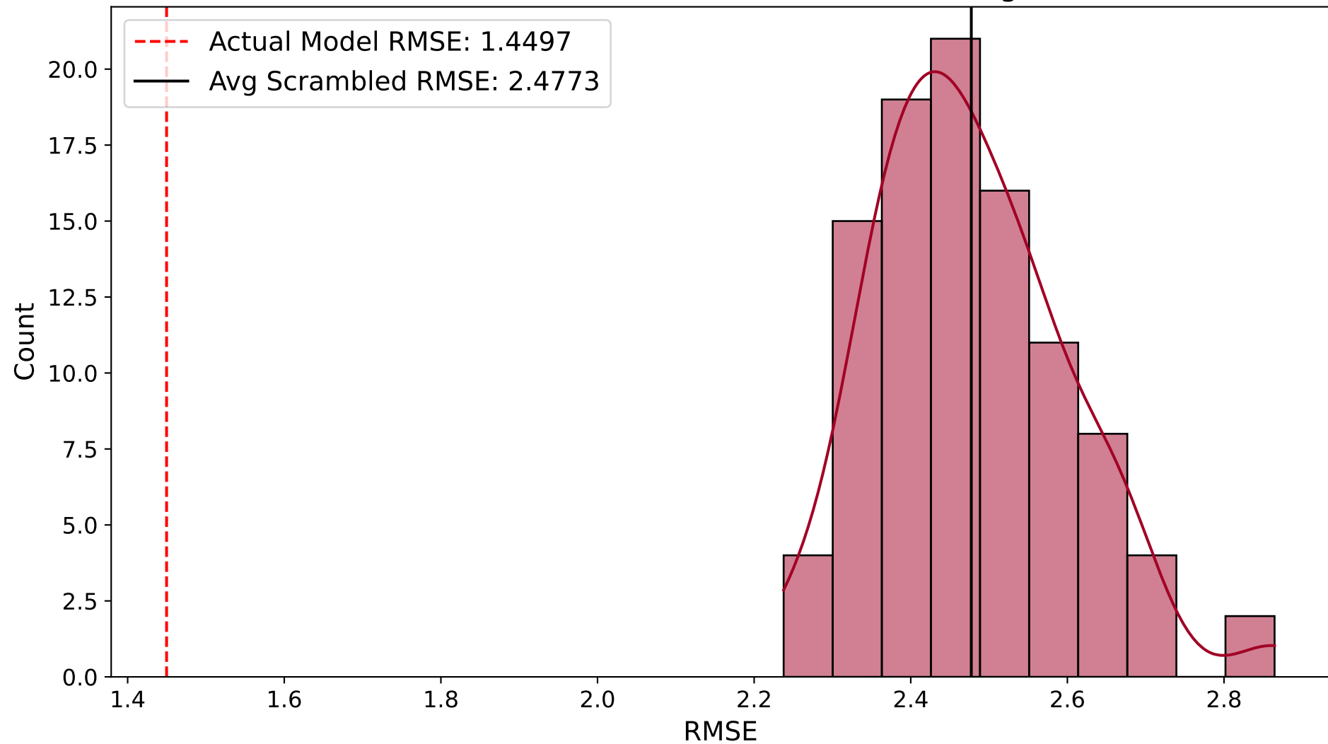
Distribution of RMSE from Y-Scrambling
