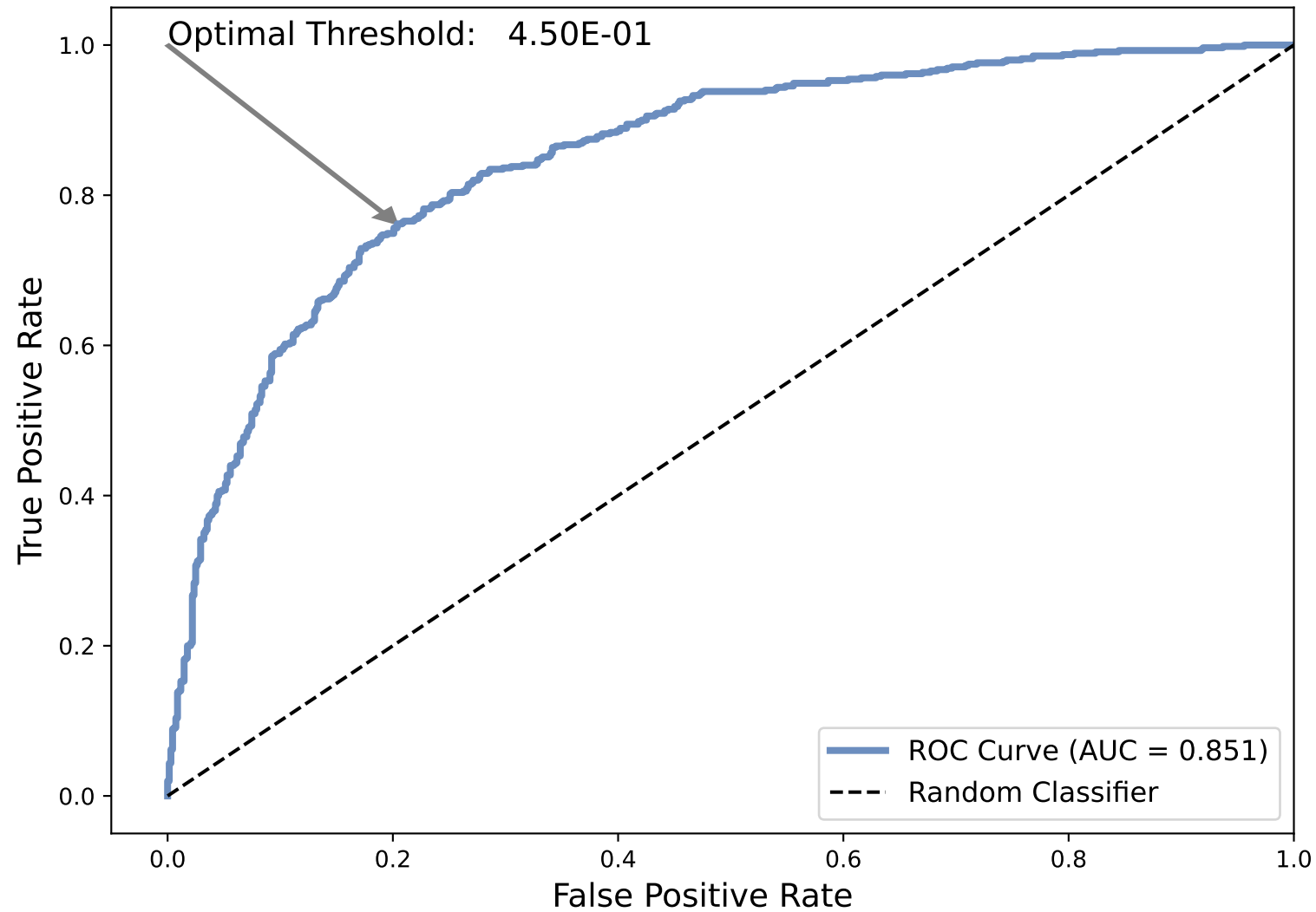
ROC Curve
