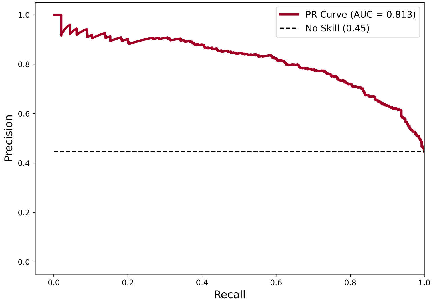
Precision-Recall Curve
