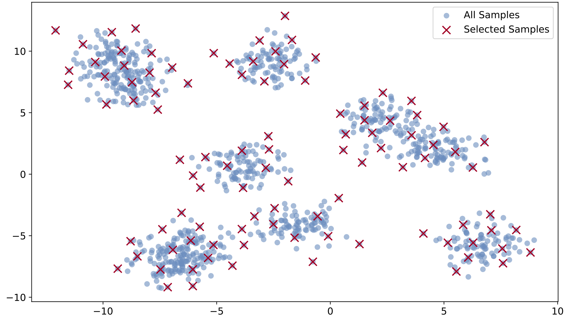
Kennard-Stone Algorithm for Representative Sample Selection
